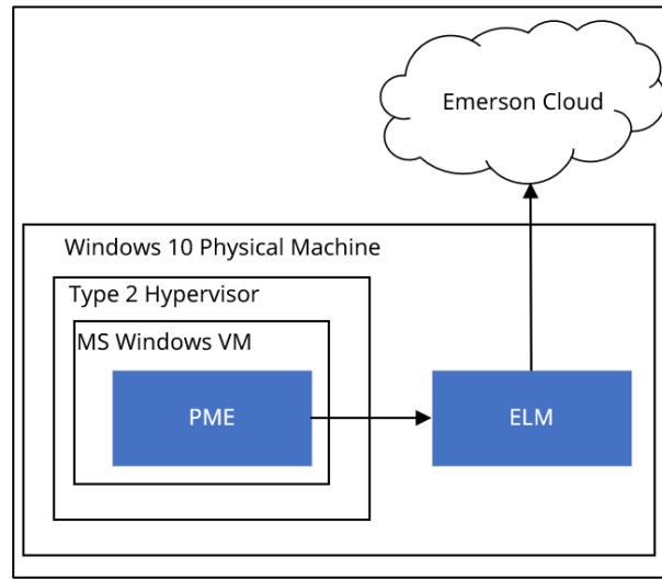
Figure 66: Type 2 Hypervisor
