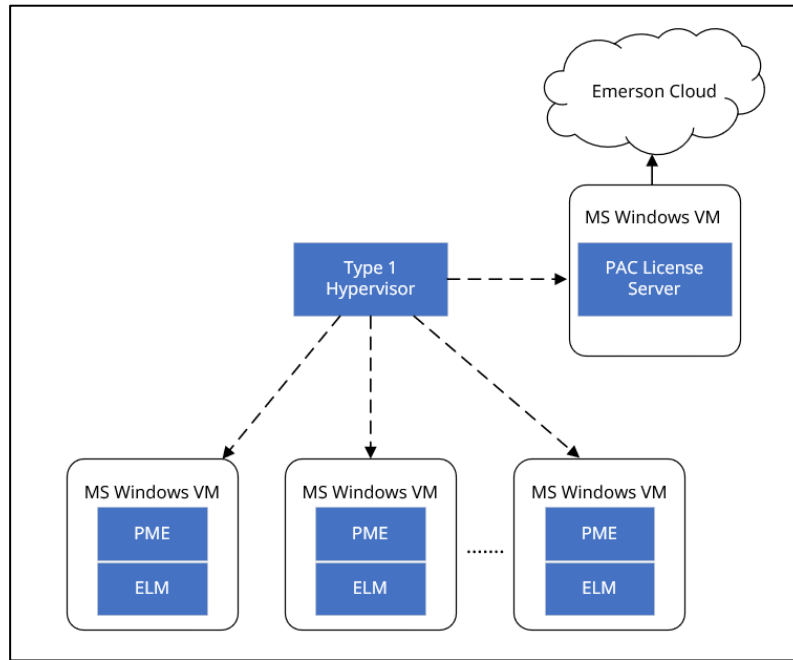
Figure 65: Type 1 Hypervisor
