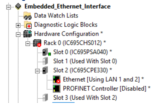
Figure 45: Embedded Ethernet Interface Configuration
