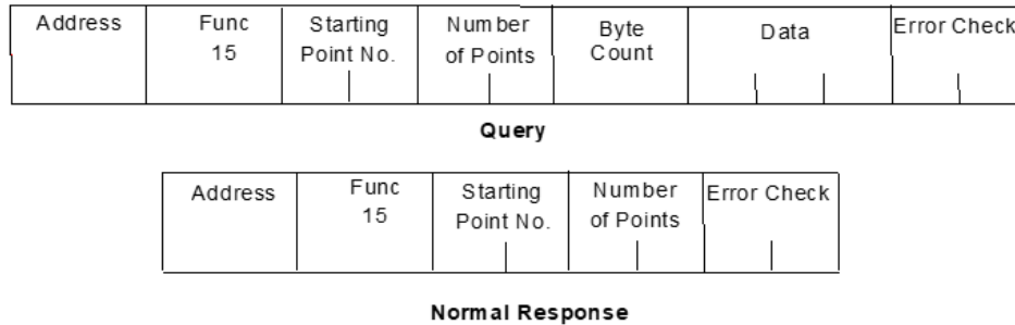
Figure 70: RTU Force Multiple Outputs Message Format
