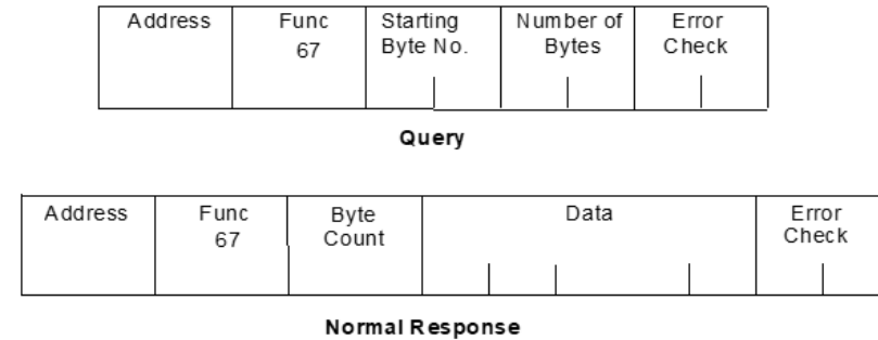
Figure 73: RTU Read Scratch Pad Memory Message Format
