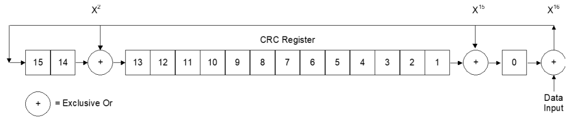
Figure 61: CRC Register Operation
