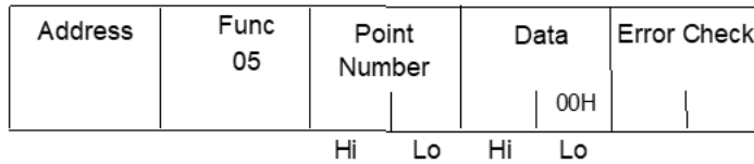
Figure 66: RTU Force Single Output Message Format
