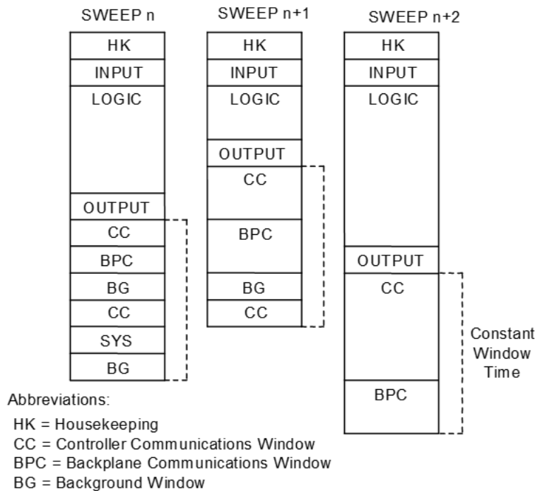
Figure 50: Typical Sweeps in Constant Window Mode
