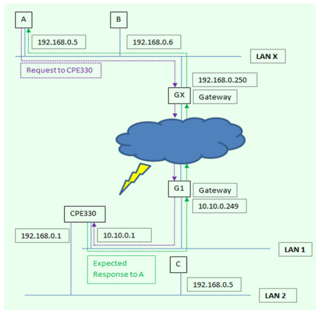
Figure 54: Expected Response Path
