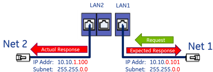
Figure 53: CPE330 Overlapping Local IP Subnet Example
