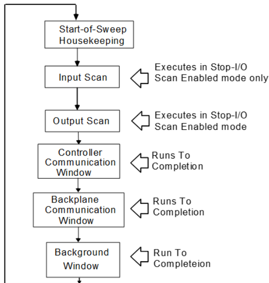
Figure 51: CPU Sweep in Stop-I/O Disabled and Stop-I/O Enabled Modes
