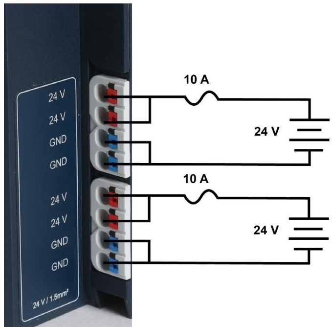
Figure 34: Power Feed Maximum Current Draw
