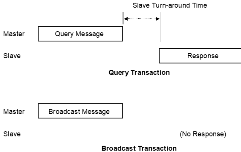
Figure 58: RTU Message Transactions
