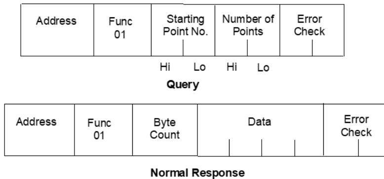
Figure 62: RTU Read Output Table Message Format
