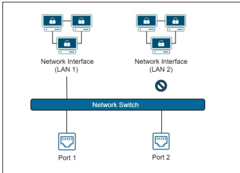
Figure 36: Single-LAN Mode
