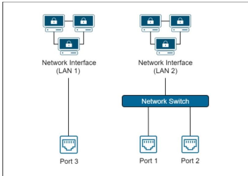
Figure 38: Network Configuration
