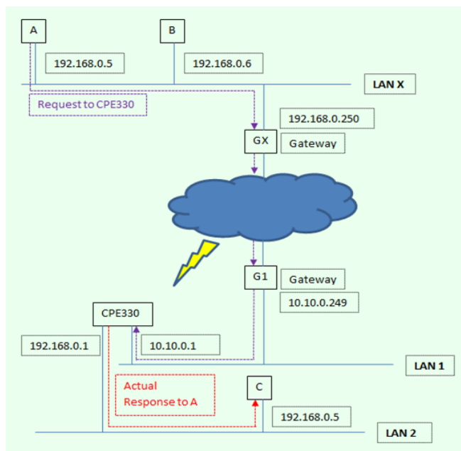
Figure 55: Actual Response Path
