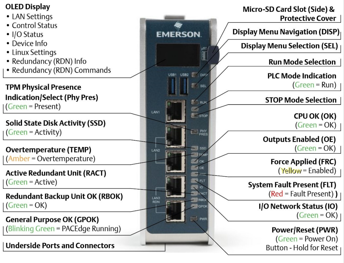
Figure 3: CPE400/CPL410/ Front View and Features
