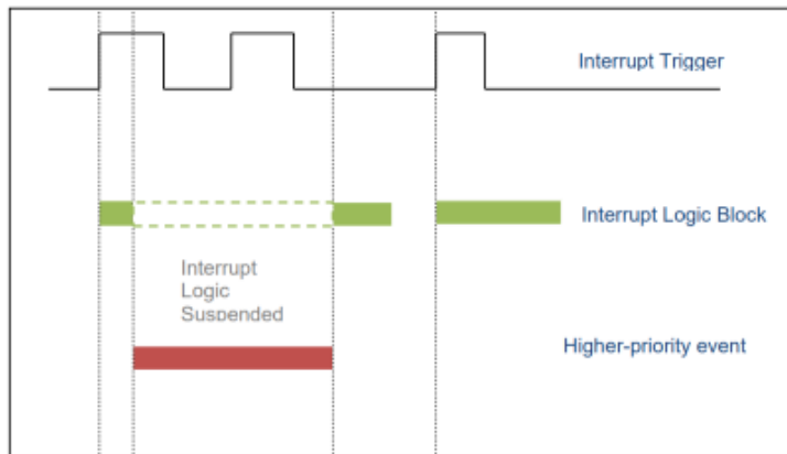
Figure 75: Interrupt Execution Considerations
