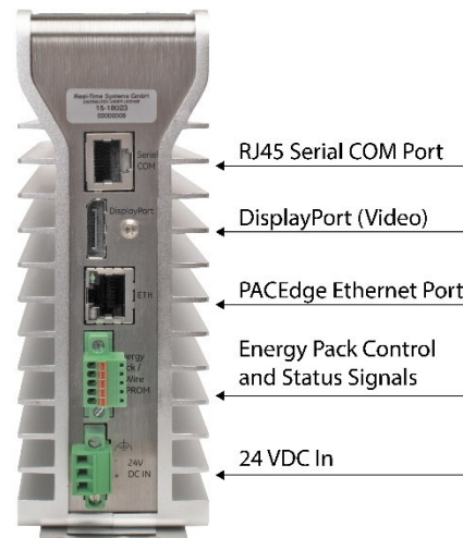
Figure 5: Underside Ports & Connectors
