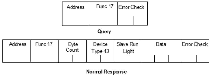
Figure 72: RTU Report Device Type Message Format
