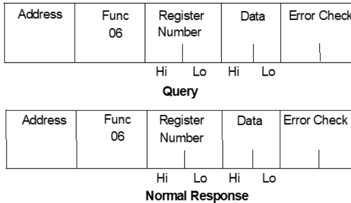
Figure 67: RTU Preset Single Register Message Format
