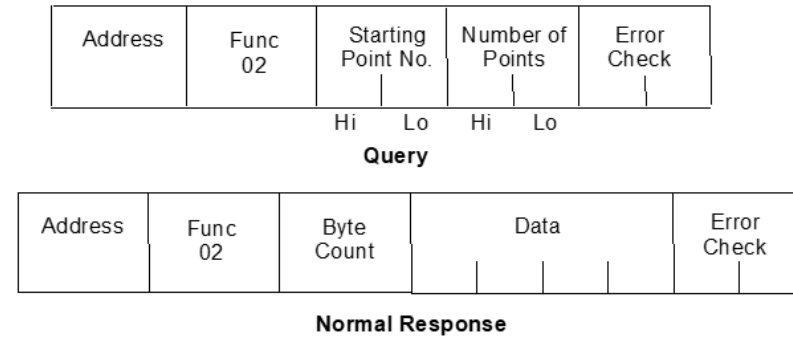
Figure 63: RTU Read Input Table Message Format
