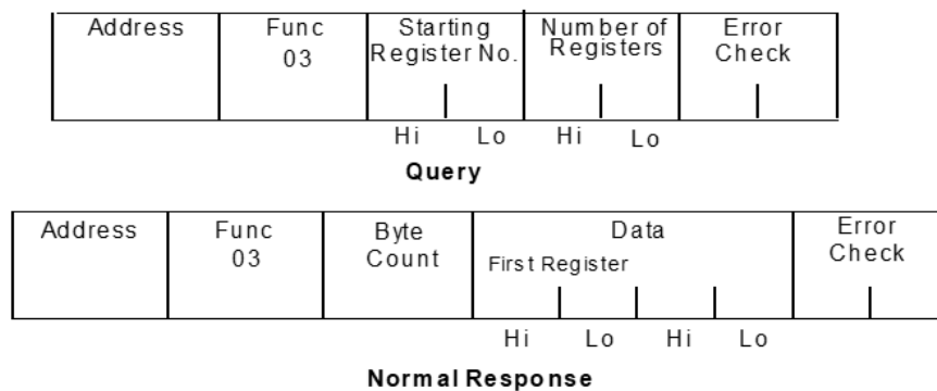
Figure 64: RTU Read Registers Message Format
