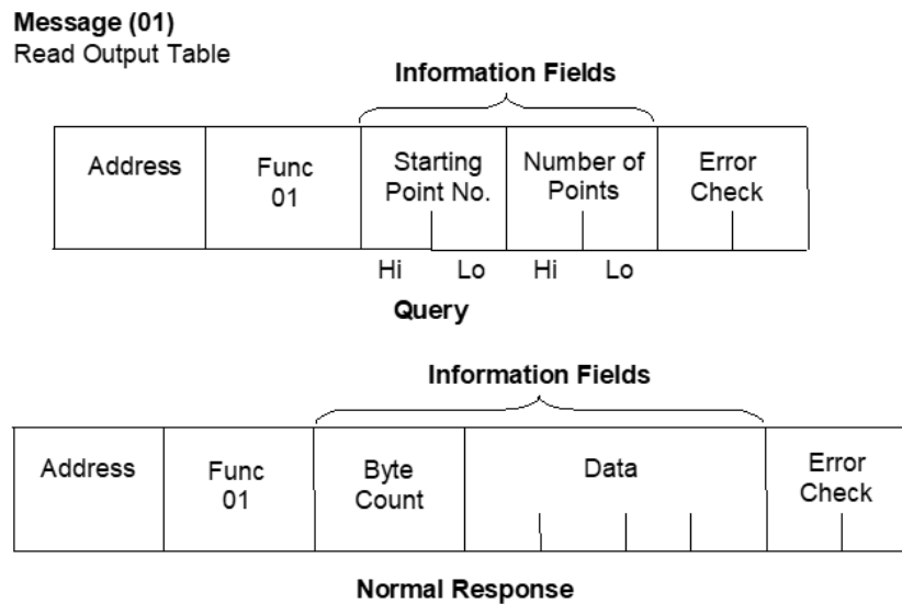
Figure 60: RTU Read Output Table Example
