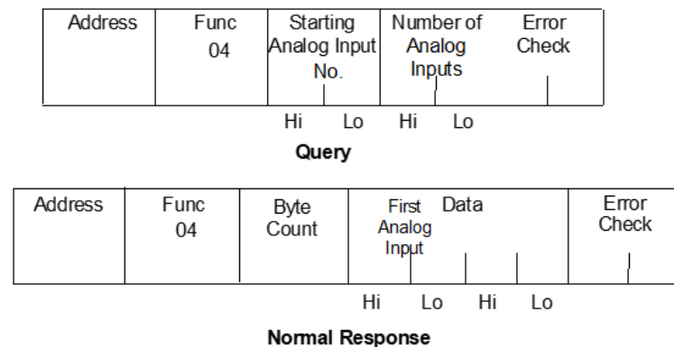
Figure 65: RTU Read Analog Inputs Message Format
