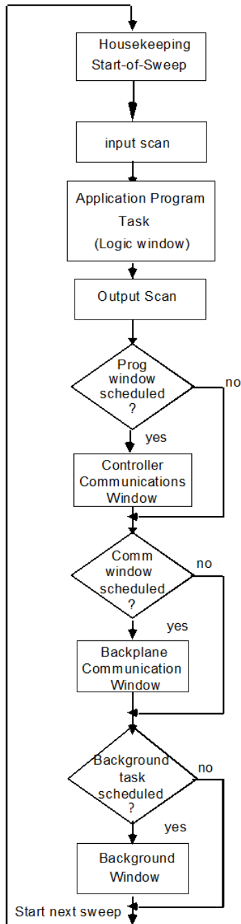
Figure 47: Major Phases of a Typical CPU Sweep
