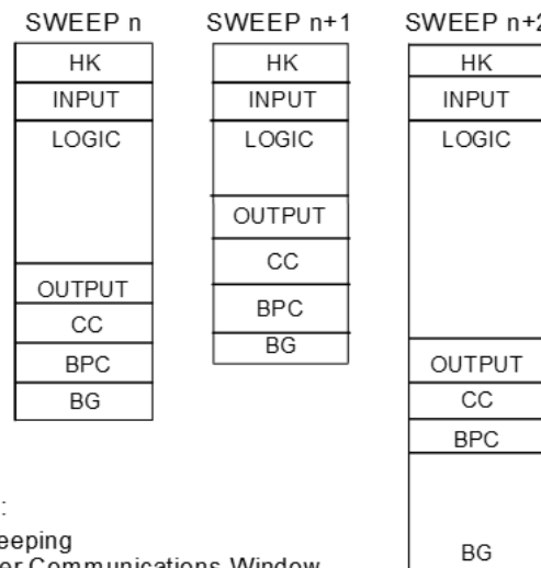
Figure 48: Typical Sweeps in Normal Sweep Mode
