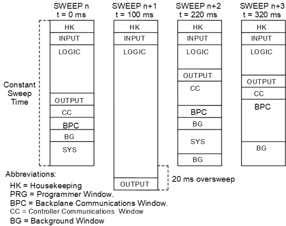
Figure 49: Typical Sweeps in Constant Sweep Mode
