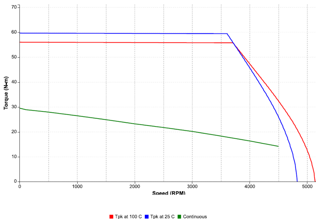
Figure 77: Speed-torque performance of an IC830M72Q motor with an IC830DP02407 drive at 400 VAC
