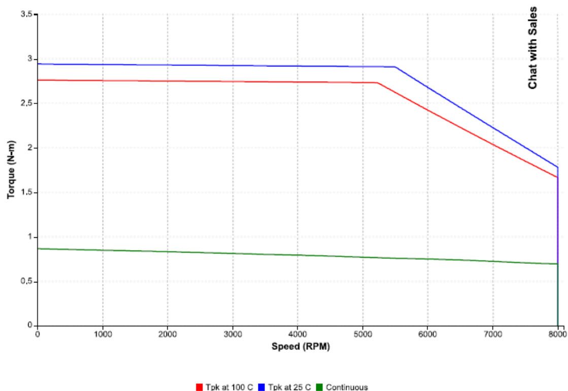
Figure 18: Speed-torque performance of an IC830M22E motor with an IC830DP00606 drive at 230 VAC
