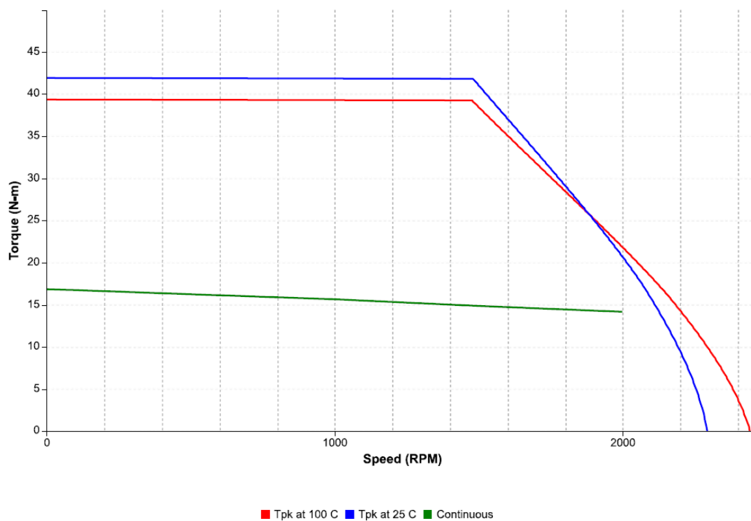
Figure 61: Speed-torque performance of an IC830M63L motor with an IC830DP01206 drive at 230 VAC
