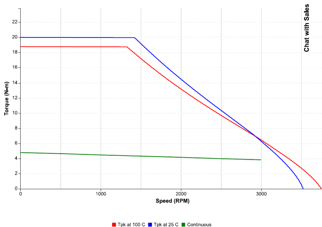
Figure 40: Speed-torque performance of an IC830M43G motor with an IC830DP01206 drive at 230 VAC
