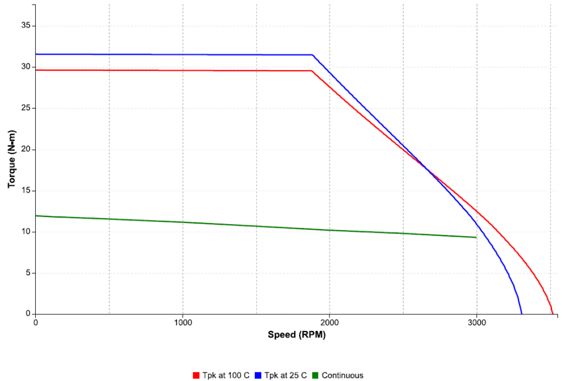
Figure 49: Speed-torque performance of an IC830M62H motor with an IC830DP00607 drive at 480 VAC
