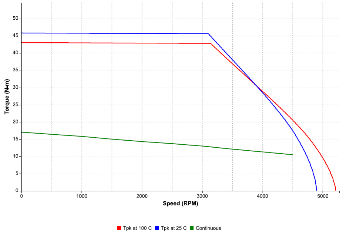
Figure 68: Speed-torque performance of an IC830M63M motor with an IC830DP02407 drive at 400 VAC
