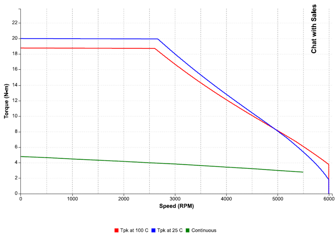
Figure 42: Speed-torque performance of an IC830M43G motor with an IC830DP01207 drive at 400 VAC
