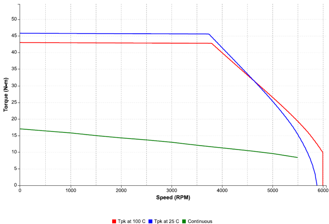
Figure 69: Speed-torque performance of an IC830M63M motor with an IC830DP02407 drive at 480 VAC
