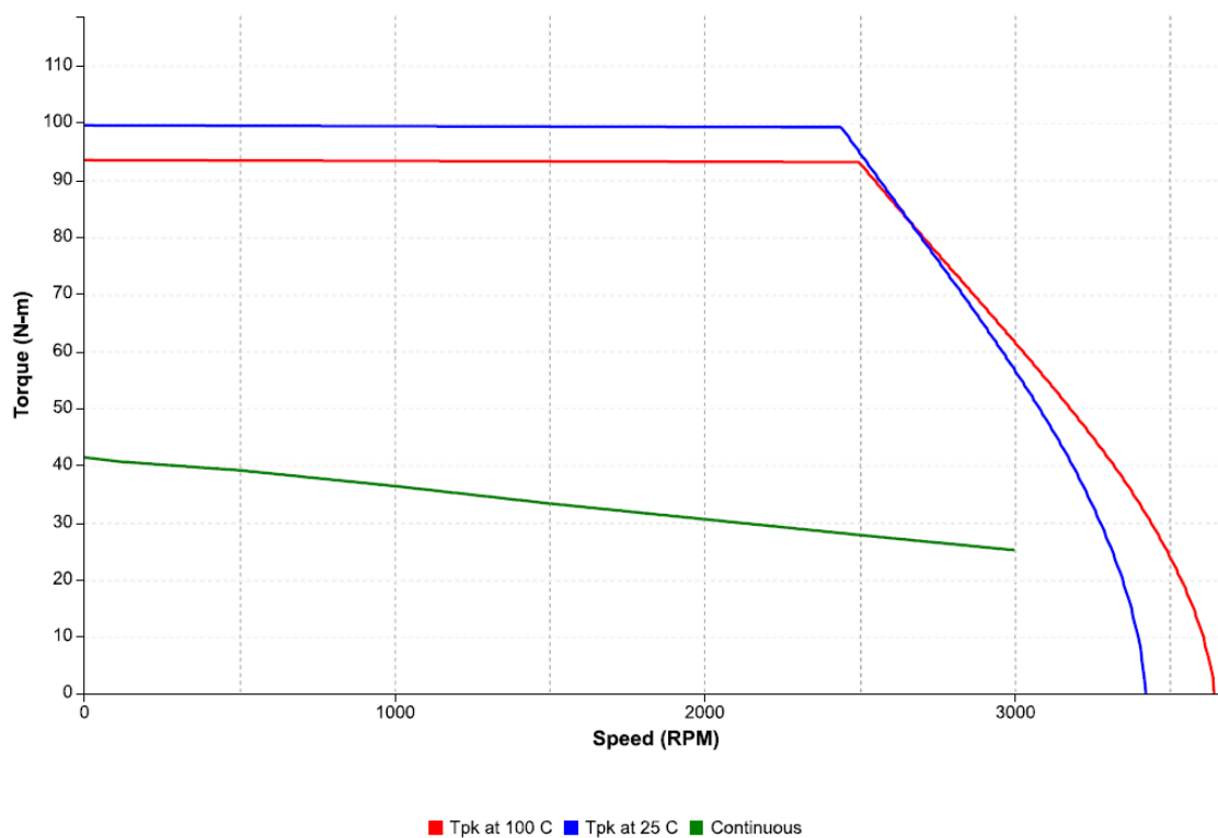
Figure 82: Speed-torque performance of an IC830M73P motor with an IC830DP02407 drive at 480 VAC
