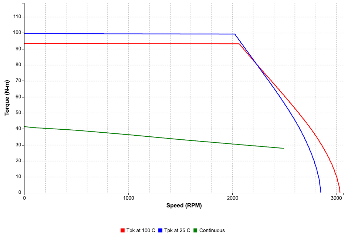
Figure 81: Speed-torque performance of an IC830M73P motor with an IC830DP02407 drive at 400 VAC
