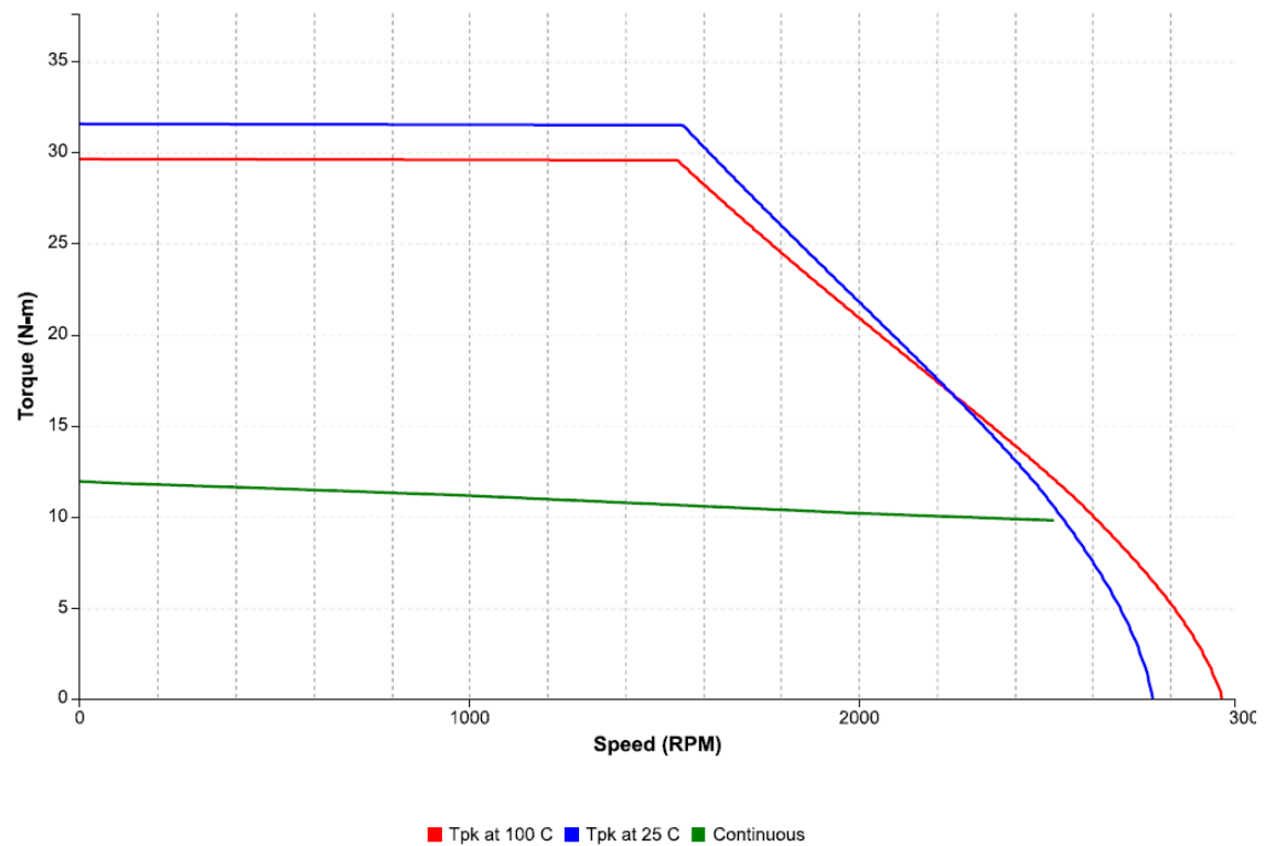
Figure 48: Speed-torque performance of an IC830M62H motor with an IC830DP00607 drive at 400 VAC
