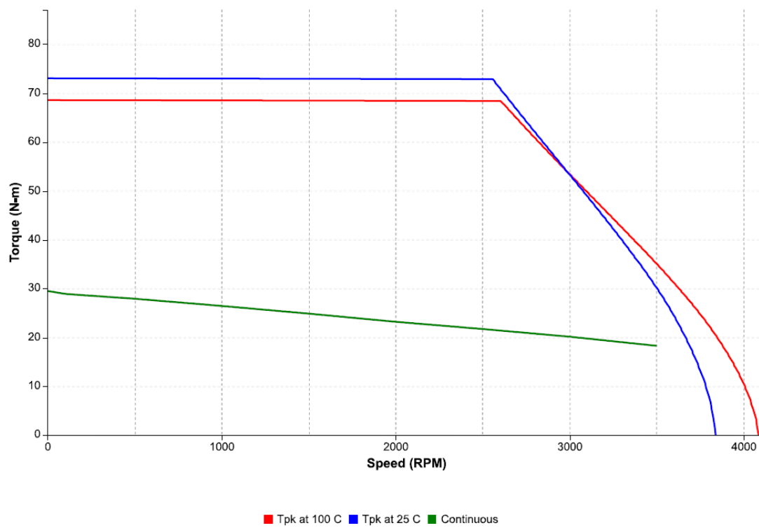
Figure 74: Speed-torque performance of an IC830M72P motor with an IC830DP02407 drive at 400 VAC
