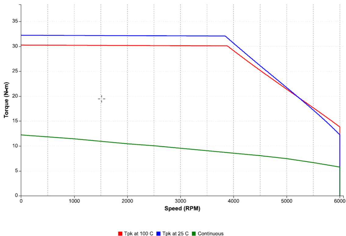
Figure 59: Speed-torque performance of an IC830M62M motor at 400 VAC with an IC830DP02407 drive at 480 VAC
