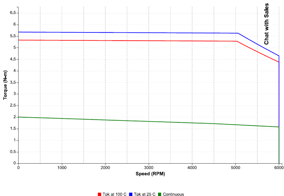
Figure 25: Speed-torque performance of an IC830M41E motor with an IC830DP00607 drive at 480 VAC
