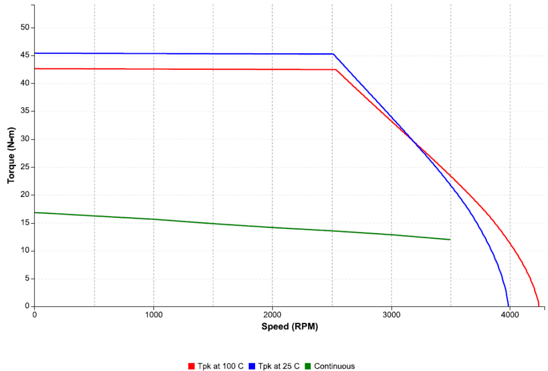
Figure 64: Speed-torque performance of an IC830M63L motor with an IC830DP02407 drive at 400 VAC
