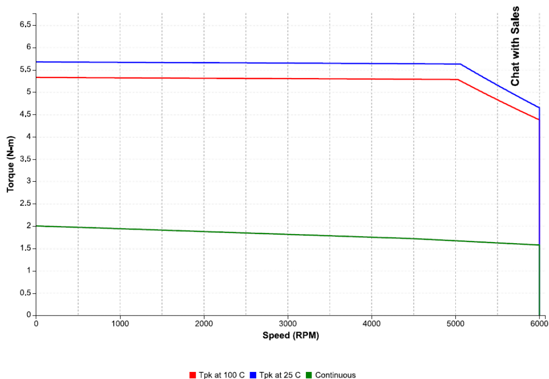
Figure 24: Speed-torque performance of an IC830M41E motor with an IC830DP00307 drive at 480 VAC
