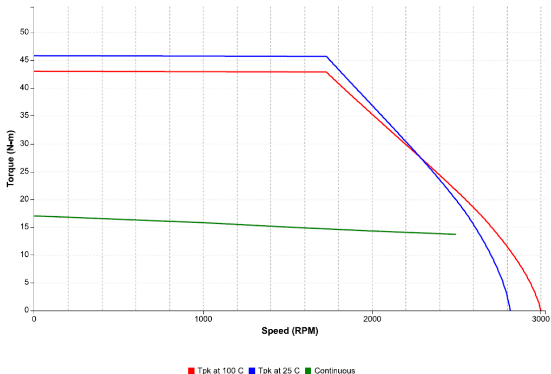
Figure 67: Speed-torque performance of an IC830M63M motor with an IC830DP02406 drive at 230 VAC
