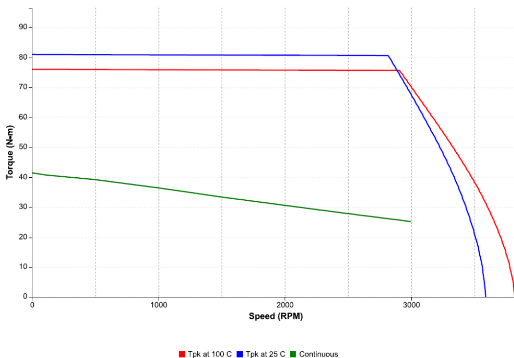
Figure 84: Speed-torque performance of an IC830M73Q motor with an IC830DP02407 drive at 400 VAC
