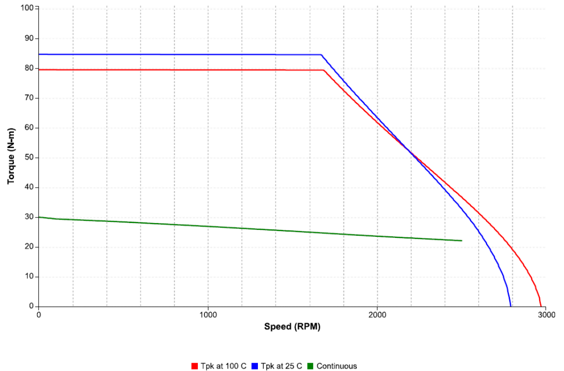
Figure 72: Speed-torque performance of an IC830M72L motor with an IC830DP02407 drive at 480 VAC
