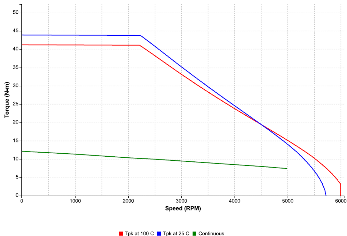
Figure 53: Speed-torque performance of an IC830M62K motor with an IC830DP02407 drive at 480 VAC
