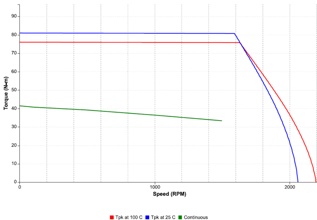
Figure 83: Speed-torque performance of an IC830M73Q motor with an IC830DP02406 drive at 230 VAC
