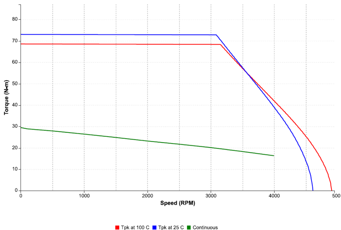
Figure 75: Speed-torque performance of an IC830M72P motor with an IC830DP02407 drive at 480 VAC
