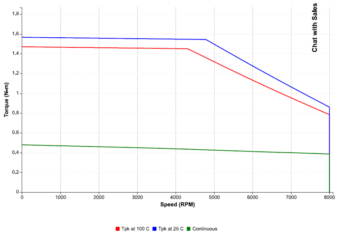
Figure 16: Speed-torque performance of an IC830M21C motor and an IC830D306 drive at 230 VAC
