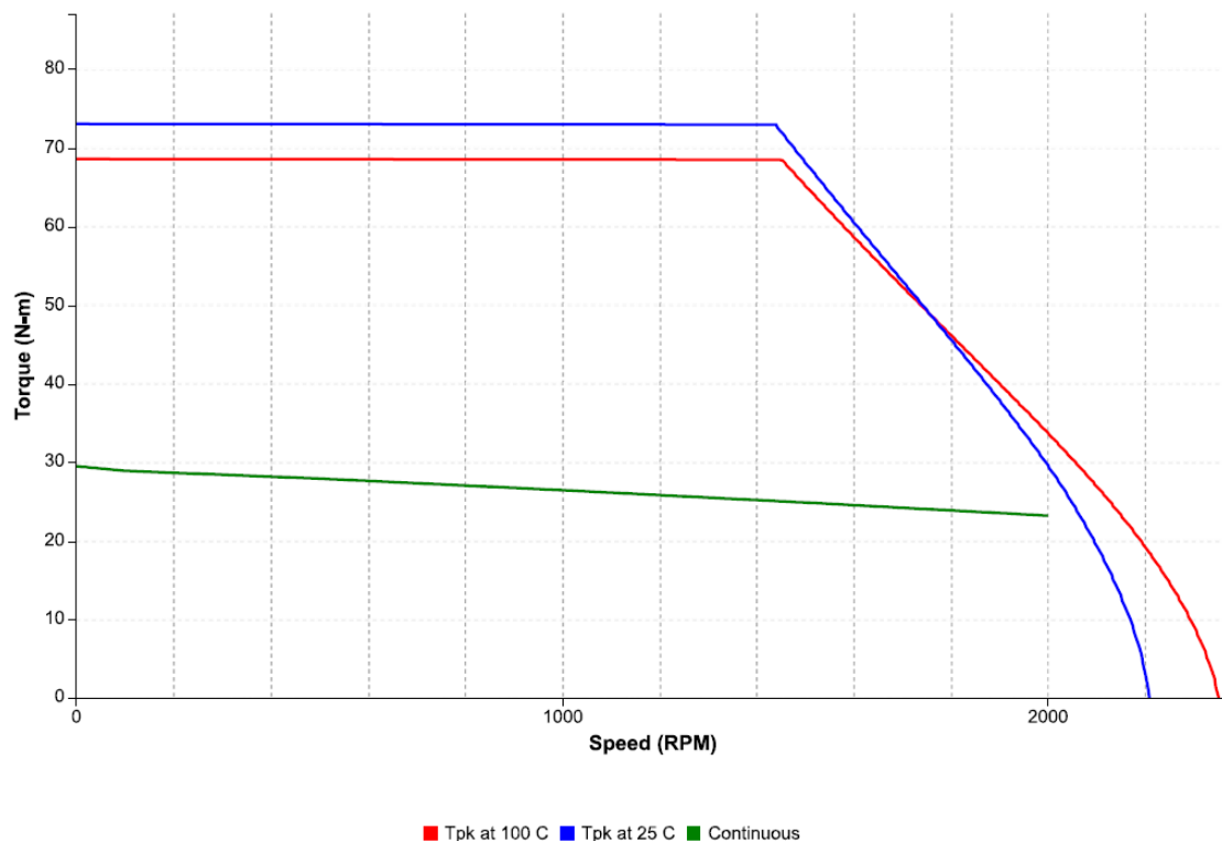
Figure 73: Speed-torque performance of an IC830M72P motor with an IC830DP02406 drive at 230 VAC
