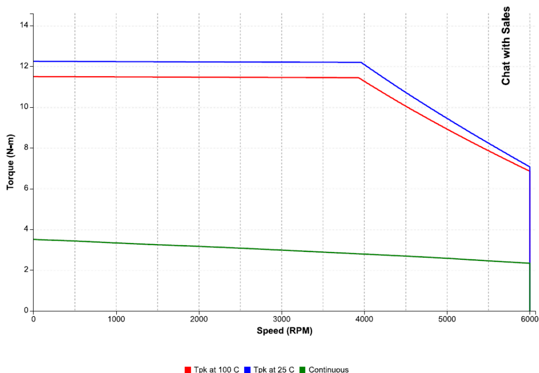
Figure 35: Speed-torque performance of an IC830M42G motor with an IC830DP01207 drive at 400 VAC
