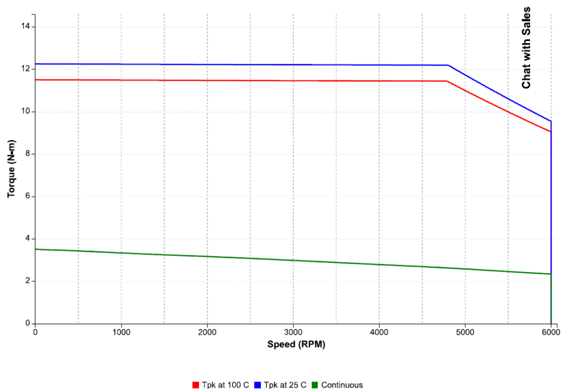
Figure 37: Speed-torque performance of an IC830M42G motor with an IC830DP01207 drive at 480 VAC
