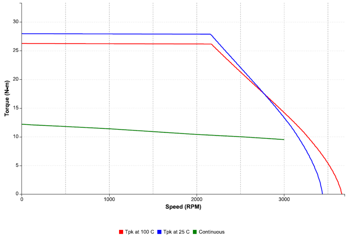
Figure 54: Speed-torque performance of an IC830M62L motor with an IC830DP02406 drive at 230 VAC
