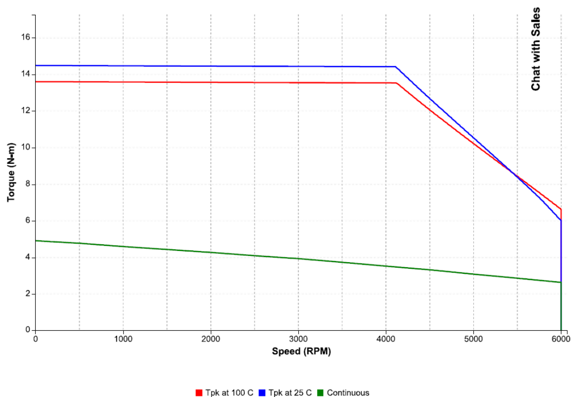
Figure 45: Speed-torque performance of an IC830M43K motor with an IC830DP01206 drive at 230 VAC
