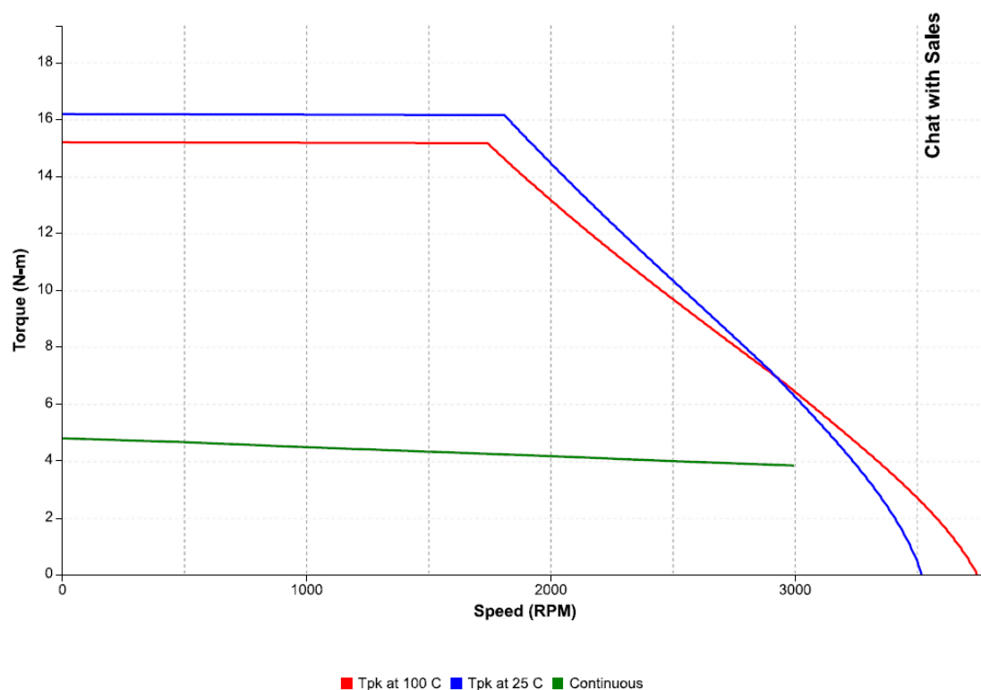
Figure 39: Speed-torque performance of an IC830M43G motor with an IC830DP00606 drive at 230 VAC
