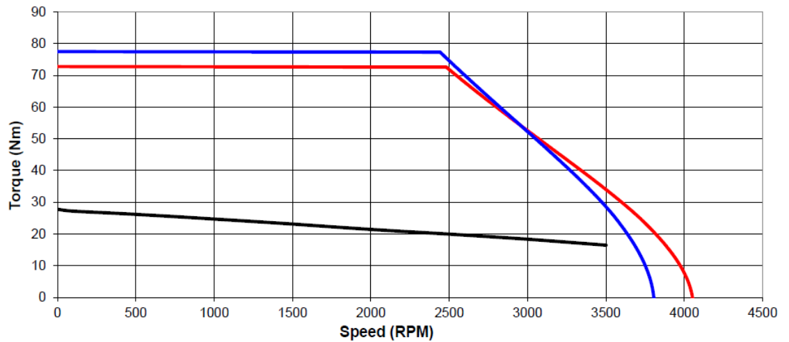
Figure 79: Speed-torque performance of an IC830M72R motor with an IC830DP02406 drive at 230 VAC
