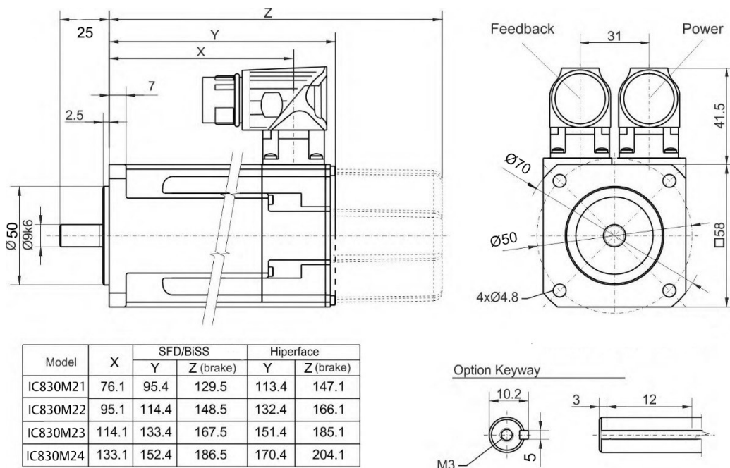
Figure 9: Radial/axial forces at shaft end (CK Flanges)
