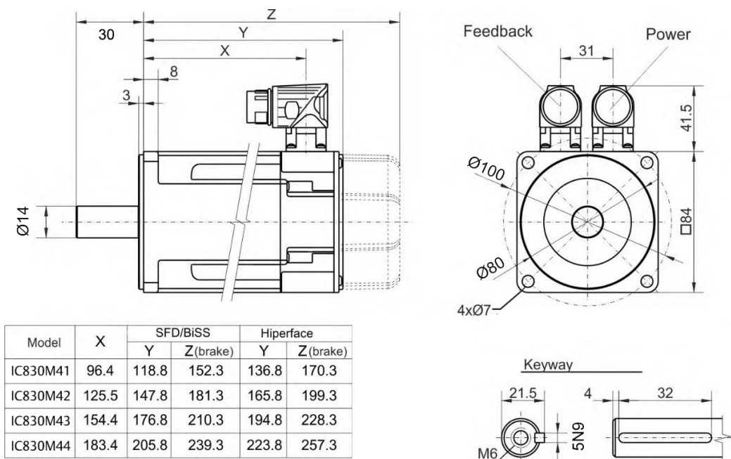
Figure 10: Dimensions with SpeedTec Ready connectors
