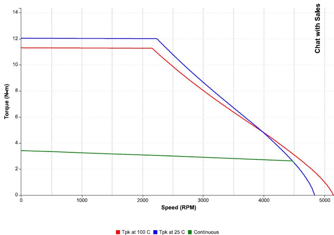
Figure 29: Speed-torque performance of an IC830M42E motor with an IC830DP00607 drive at 400 VAC
