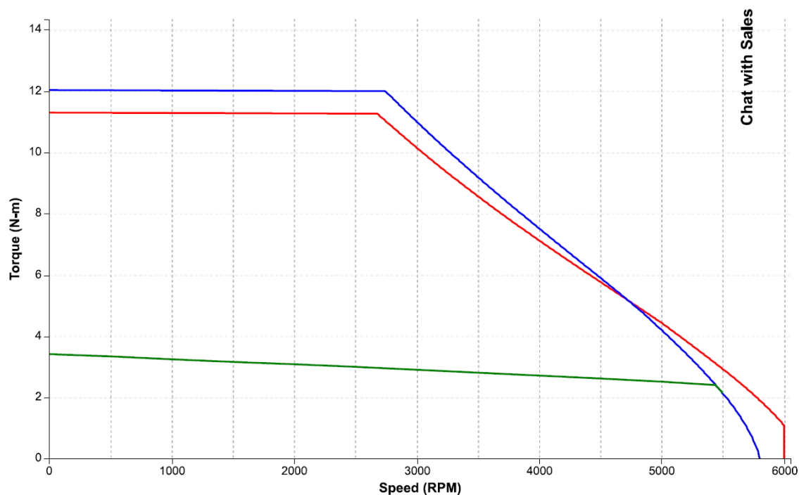
Figure 32: Speed-torque performance of an IC830M42G motor with an IC830DP00606 drive at 230 VAC
