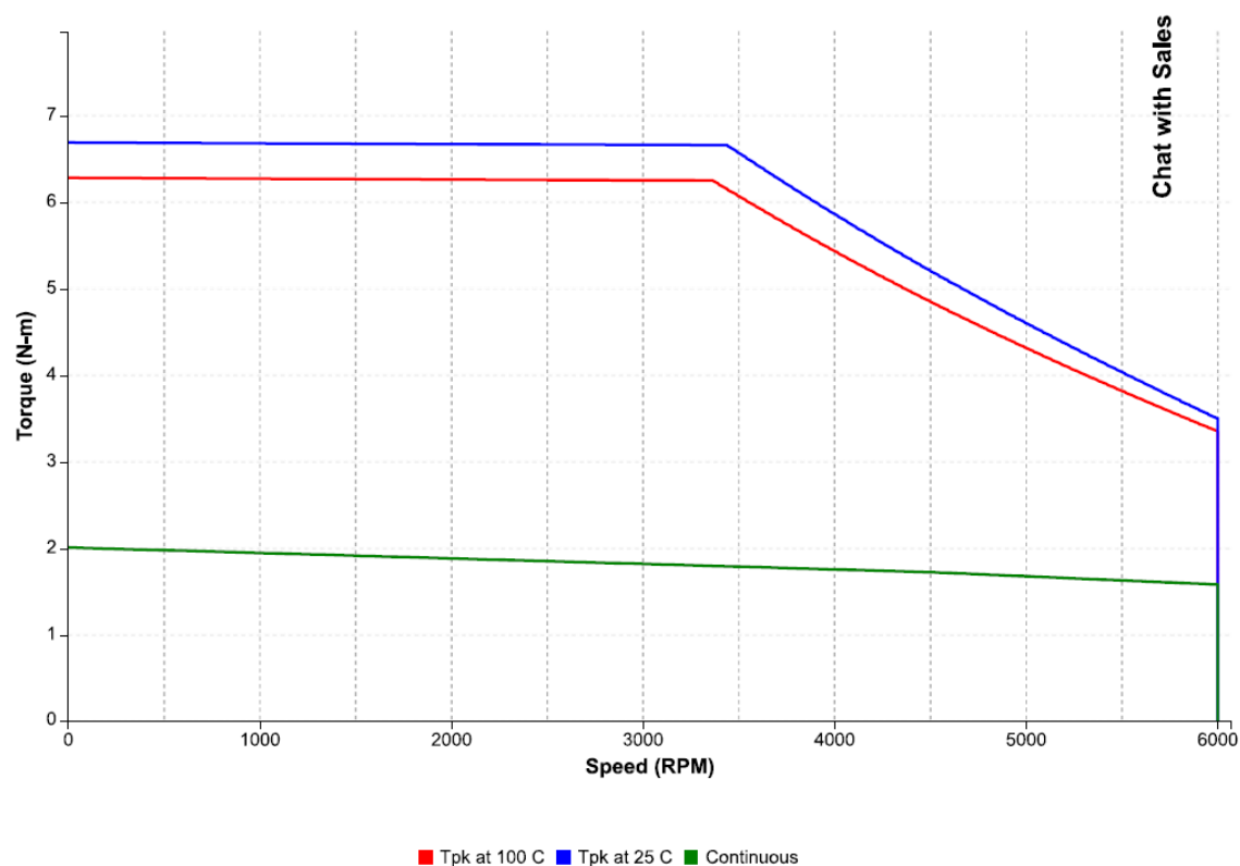
Figure 23: Speed-torque performance of an IC830M41E motor with an IC830DP00607 drive at 400 VAC
