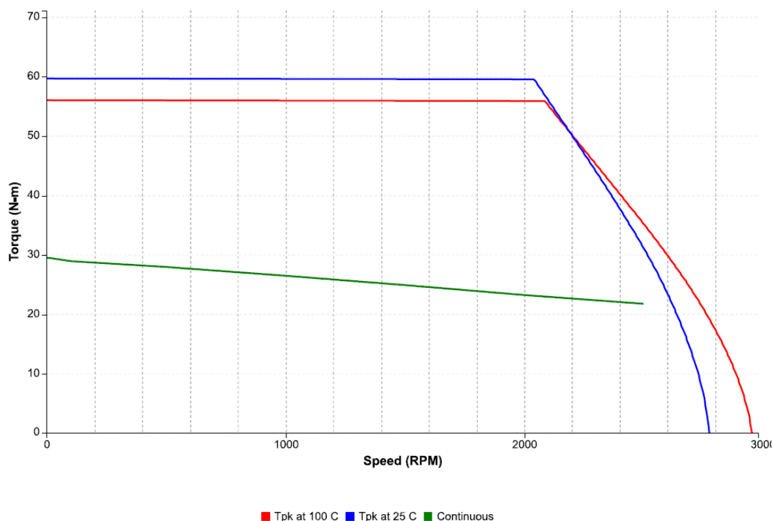
Figure 76: Speed-torque performance of an IC830M72Q motor with an IC830DP02406 drive at 230 VAC
