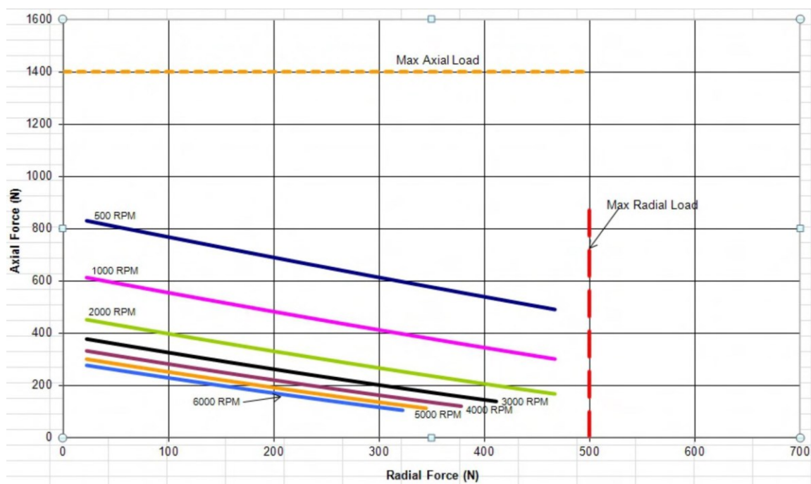
Figure 11: Radial/axial forces at shaft end
