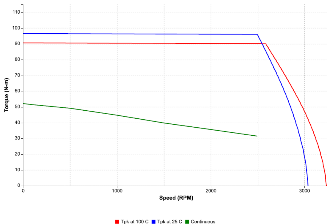
Figure 87: Speed-torque performance of an IC830M74Q motor with an IC830DP02407 drive at 400 VAC
