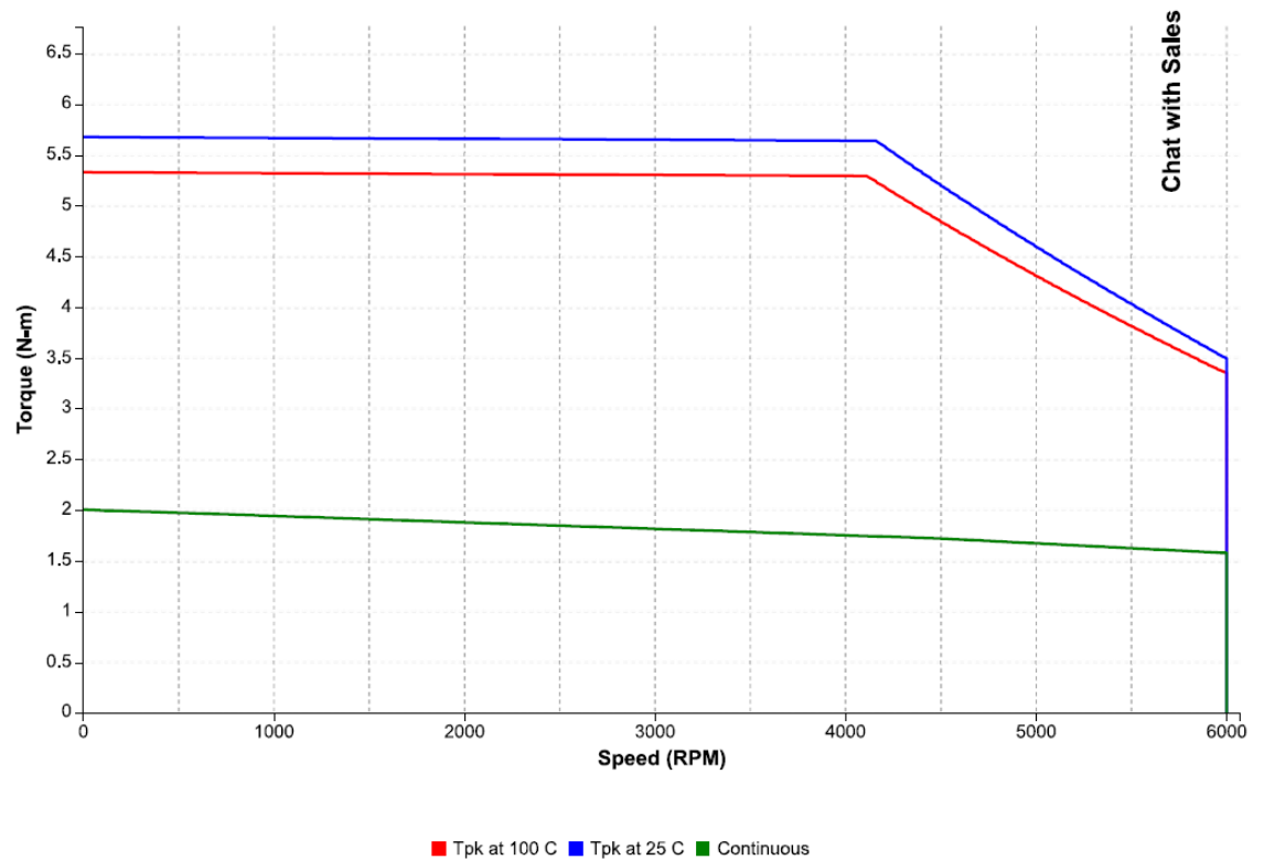
Figure 22: Speed-torque performance of an IC830M41E motor with an IC830DP00307 drive at 400 VAC
