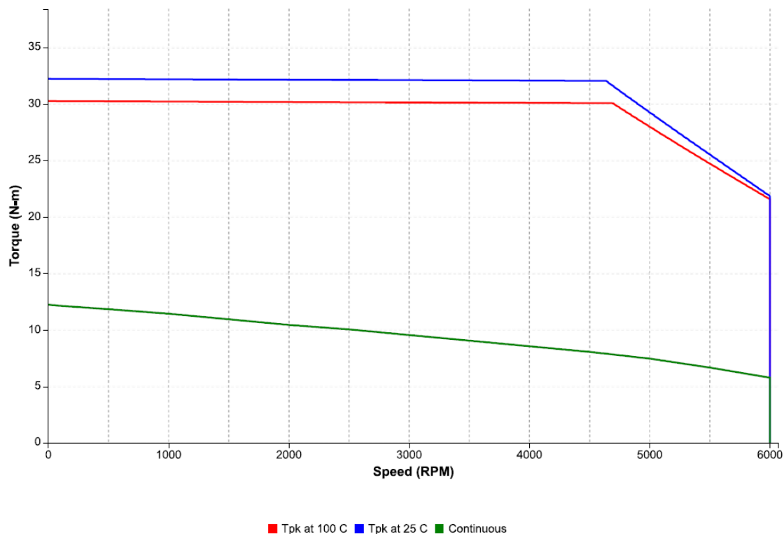
Figure 60: Speed-torque performance of an IC830M62M motor with an IC830DP02407 drive at 480 VAC
