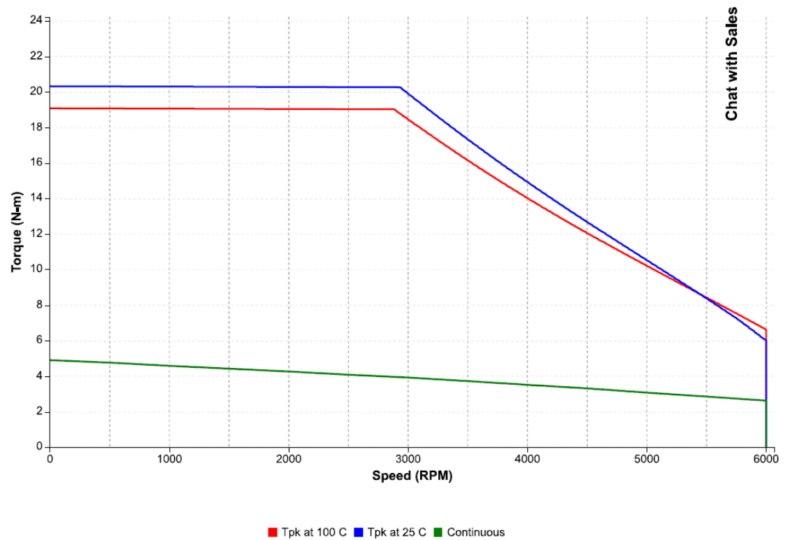
Figure 47: Speed-torque performance of an IC830M62H motor with an IC830DP00606 drive at 230 VAC
