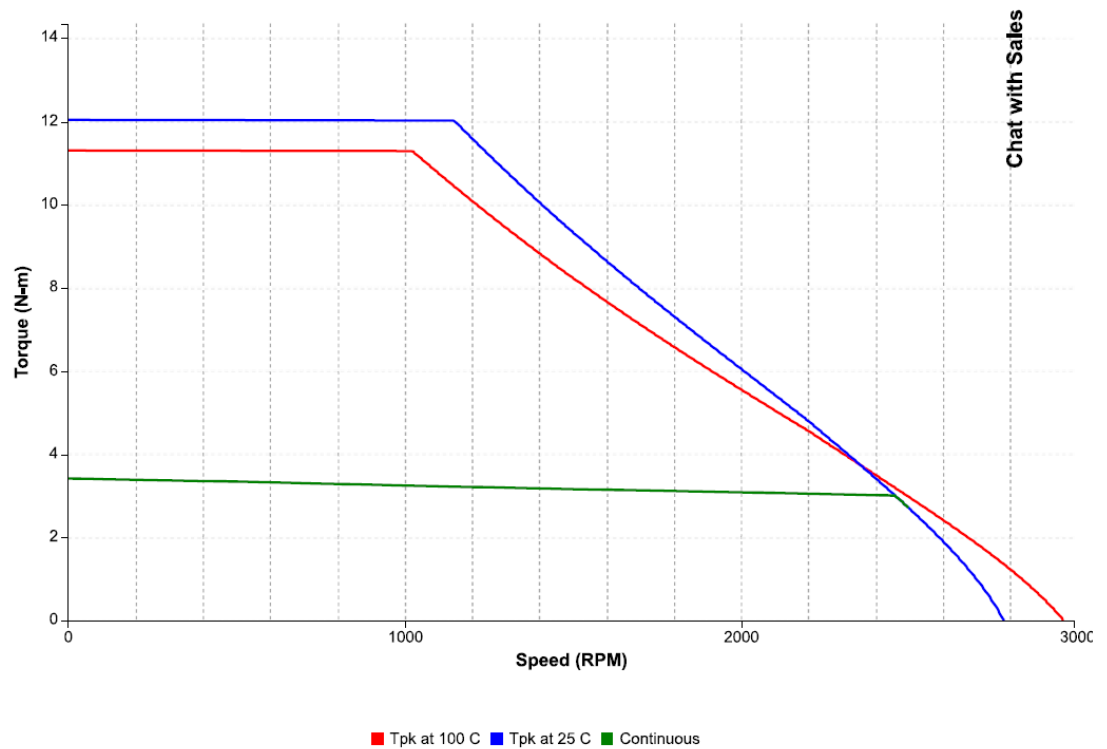
Figure 27: Speed-torque performance of an IC830M42E motor with an IC830DP00606 drive at 230 VAC
