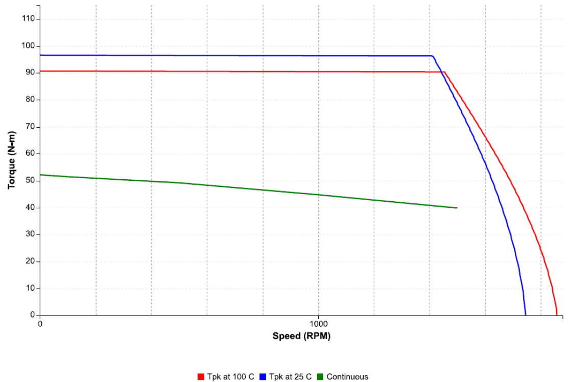
Figure 86: Speed-torque performance of an IC830M74Q motor with an IC830DP02406 drive at 230 VAC
