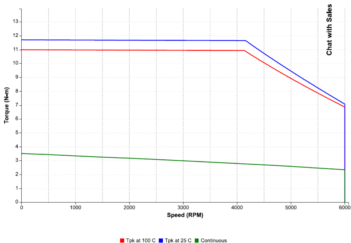
Figure 34: Speed-torque performance of an IC830M42G motor with an IC830DP00607 drive at 400 VAC
