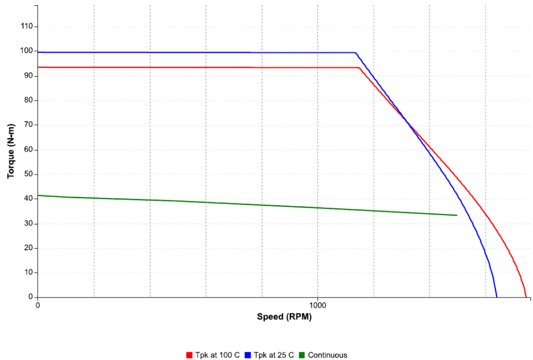
Figure 80: Speed-torque performance of an IC830M73P motor with an IC830DP02406 drive at 230 VAC
