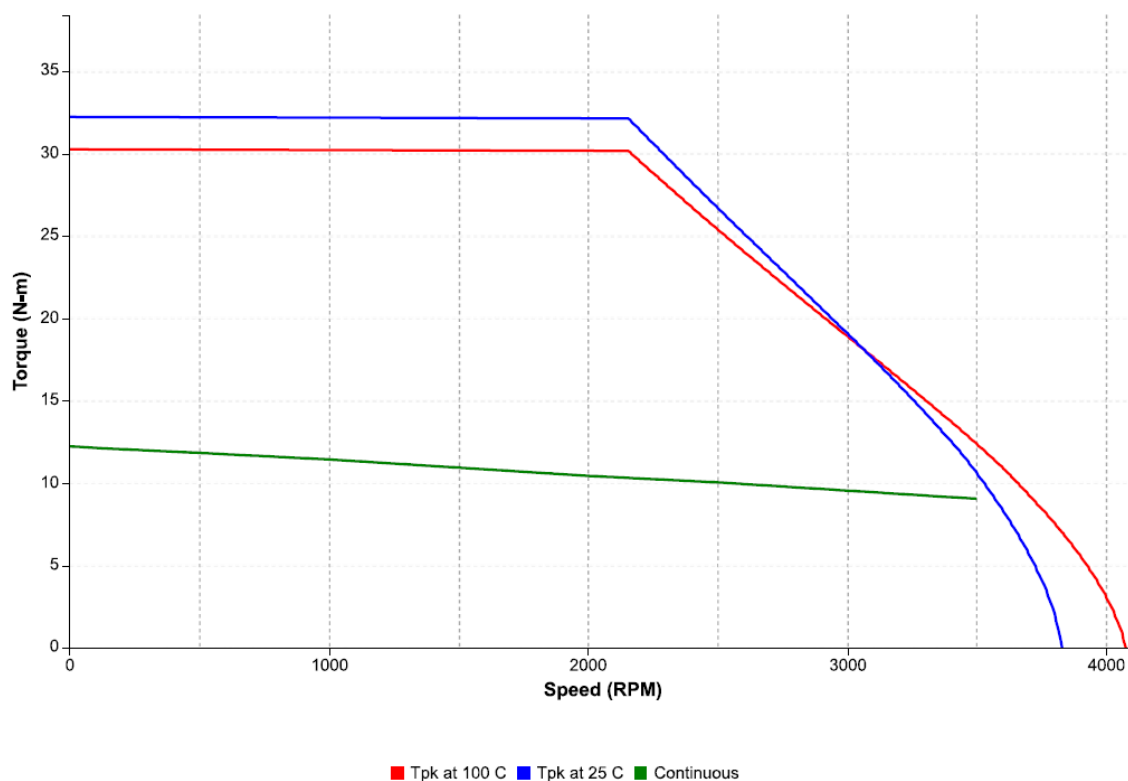
Figure 58: Speed-torque performance of an IC830M62M motor with an IC830DP02406 drive at 230 VAC
