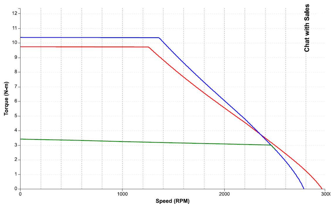
Figure 26: Speed-torque performance of an IC830M42E motor with an IC830DP00306 drive at 230 VAC
