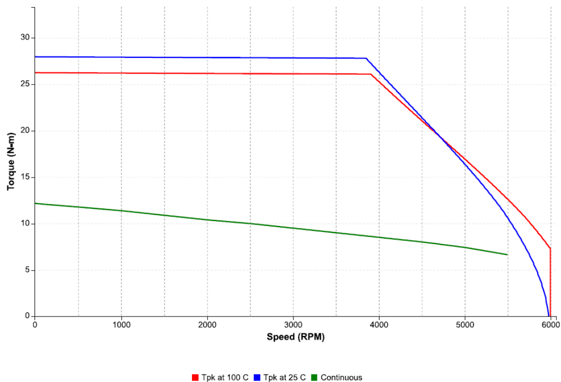
Figure 55: Speed-torque performance of an IC830M62L motor with an IC830DP02407 drive at 400 VAC
