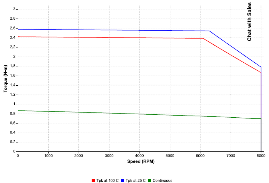
Figure 17: Speed-torque performance of an IC830M22E motor with an IC830DP00306 drive at 230 VAC
