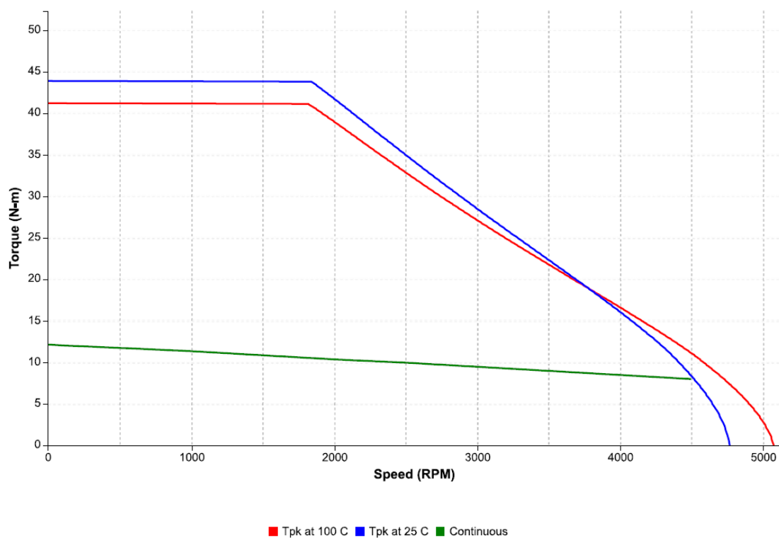
Figure 52: Speed-torque performance of an IC830M62K motor with an IC830DP02407 drive at 400 VAC
