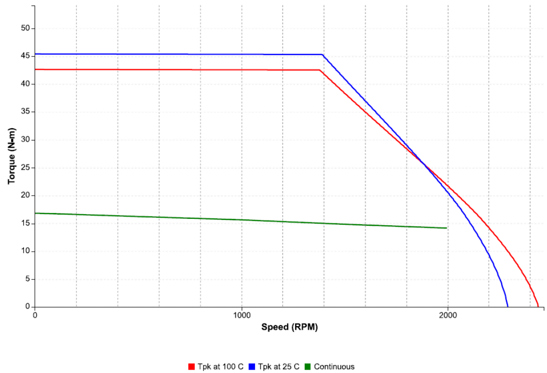
Figure 62: Speed-torque performance of an IC830M63L motor with an IC830DP02406 drive at 230 VAC
