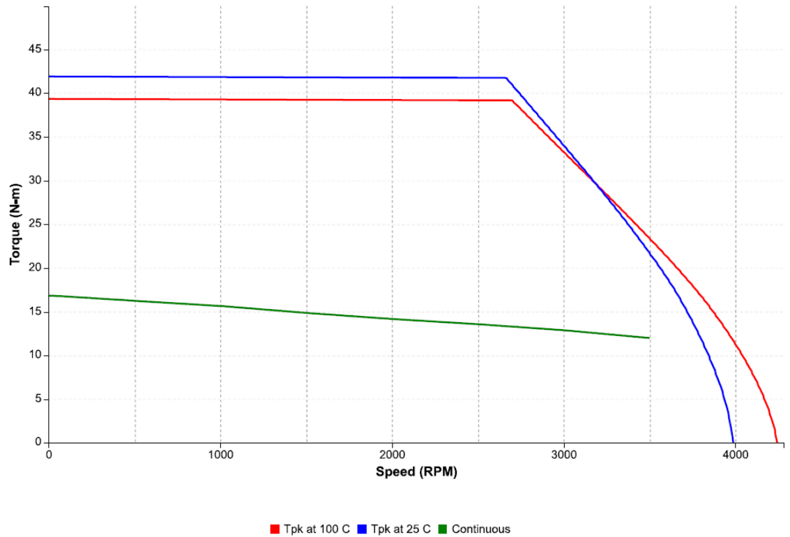
Figure 63: Speed-torque performance of an IC830M63L motor with an IC830DP01207 drive at 400 VAC
