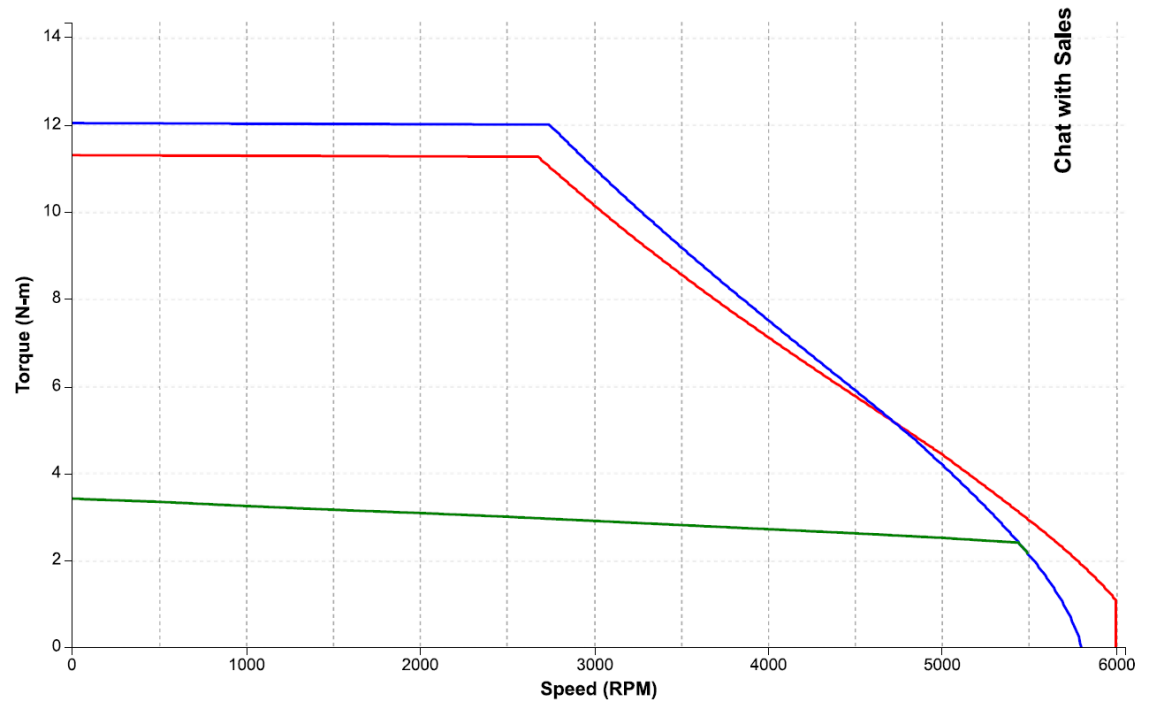
Figure 31: Speed-torque performance of an IC830M42E motor with an IC830DP00607 drive at 480 VAC
