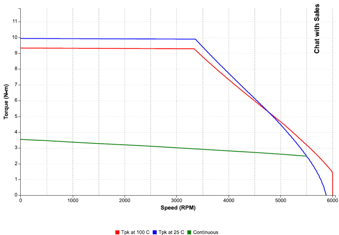
Figure 38: Speed-torque performance of an IC830M42H motor with an IC830DP00606 drive at 230 VAC
