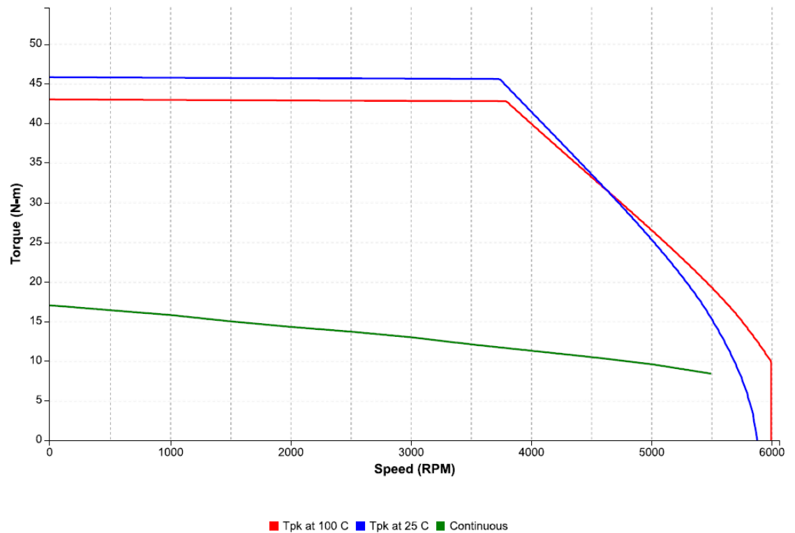
Figure 70: Speed-torque performance of an IC830M72L motor with an IC830DP01207 drive at 400 VAC
