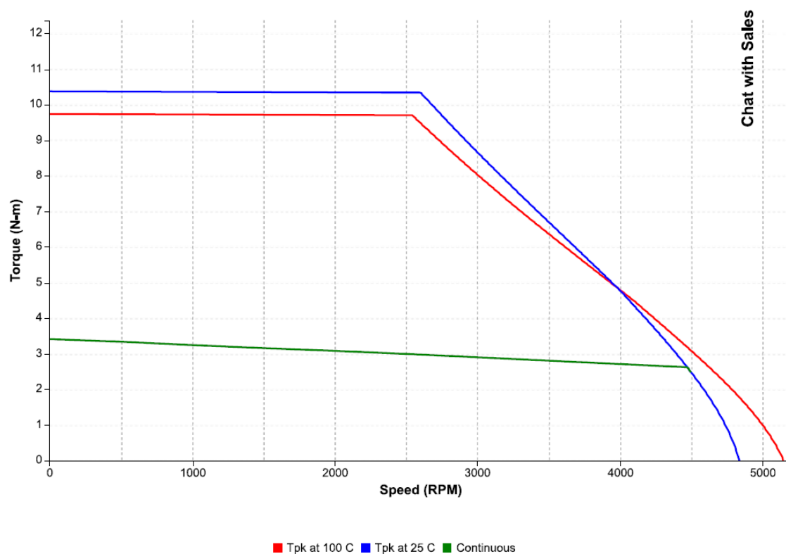
Figure 28: Speed-torque performance of an IC830M42E motor with an IC830DP00307 drive at 400 VAC
