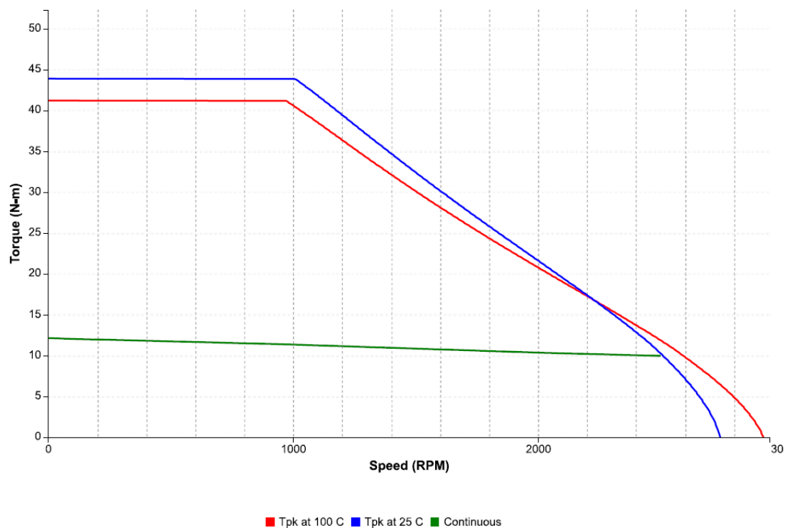
Figure 51: Speed-torque performance of an IC830M62K motor with an IC830DP02406 drive at 230 VAC
