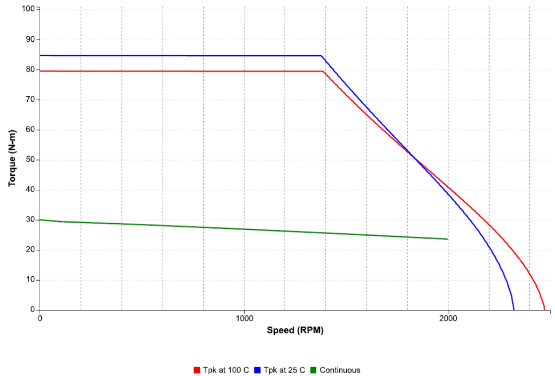
Figure 71: Speed-torque performance of an IC830M72L motor with an IC830DP02407 drive at 400 VAC
