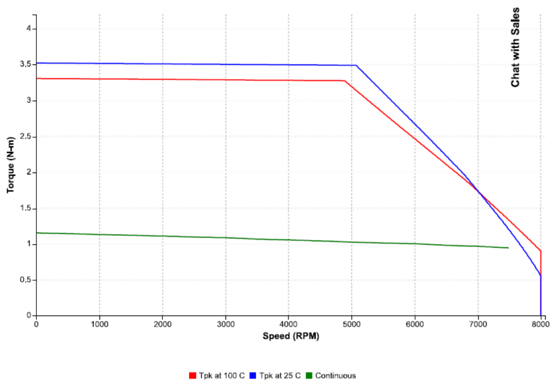
Figure 19: Speed-torque performance of an IC830M23E motor with an IC830DP00306 at 230 VAC
