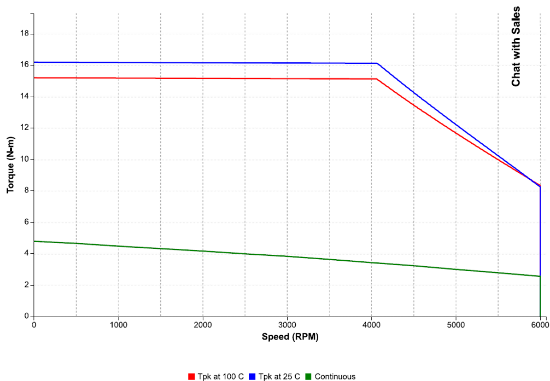
Figure 44: Speed-torque performance of an IC830M43G motor with an IC830DP00607 drive at 480 VAC
