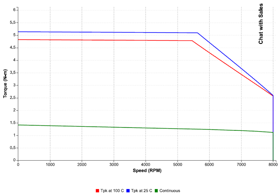
Figure 20: Speed-torque performance of an IC830M24F motor with an IC830DP00606 drive at 230 VAC
