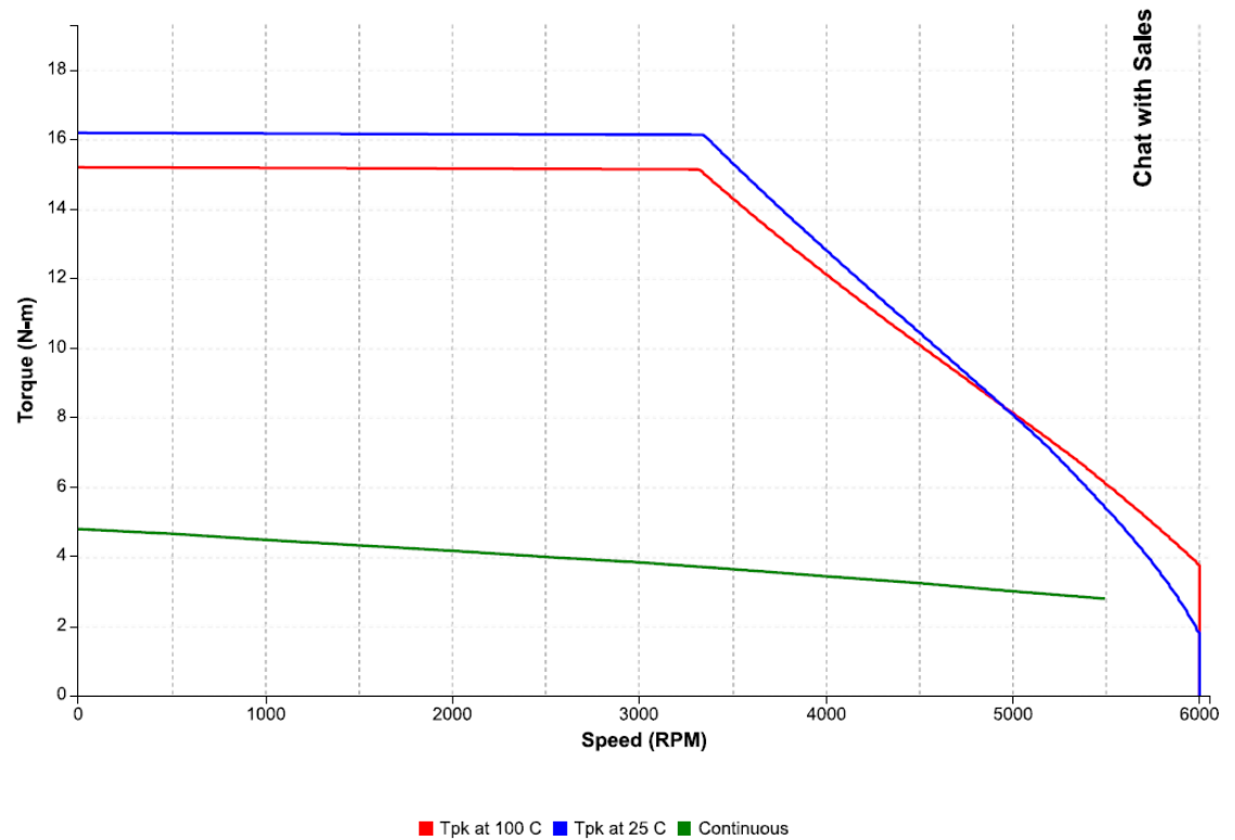
Figure 41: Speed-torque performance of an IC830M43G motor with an IC830DP00607 drive at 400 VAC
