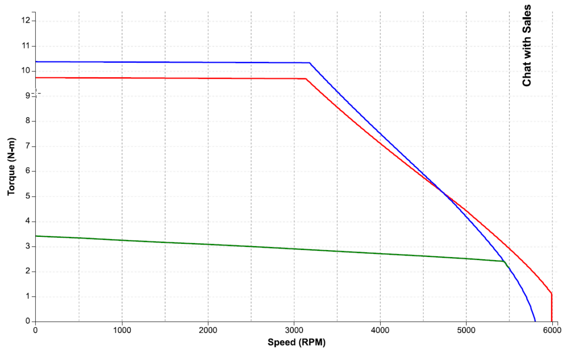
Figure 30: Speed-torque performance of an IC830M42E motor with an IC830DP00307 drive at 480 VAC
