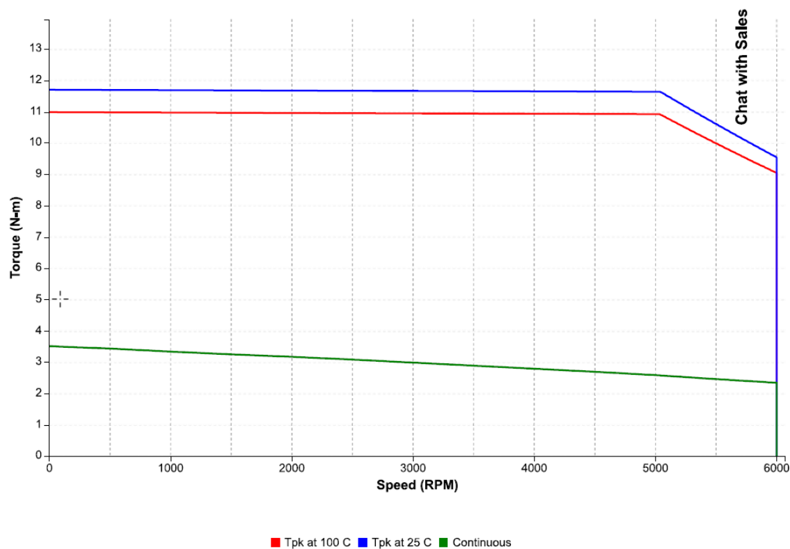
Figure 36: Speed-torque performance of an IC830M42G motor with an IC830DP00607 drive at 480 VAC
