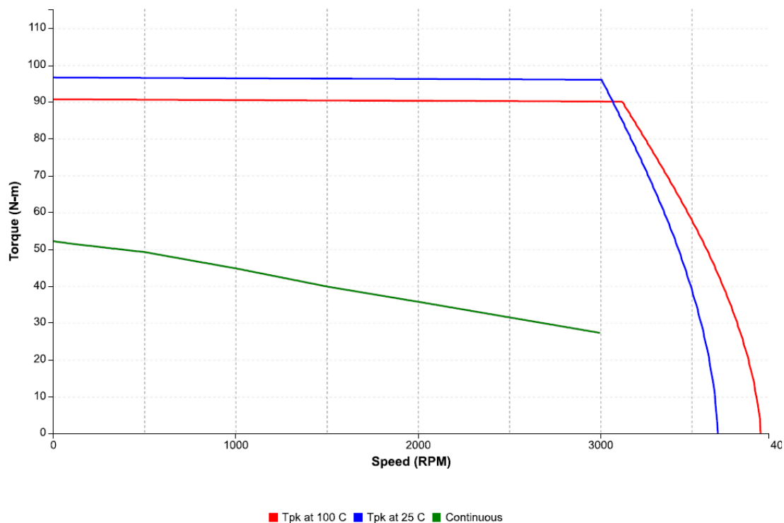
Figure 88: Speed-torque performance of an IC830M74Q motor with an IC830DP02407 drive at 480 VAC
