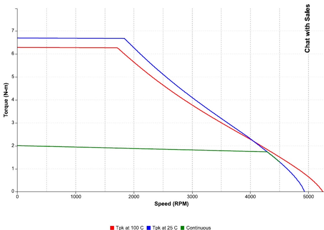
Figure 21: Speed-torque performance of an IC830M41E motor with an IC830DP00606 drive at 230 VAC
