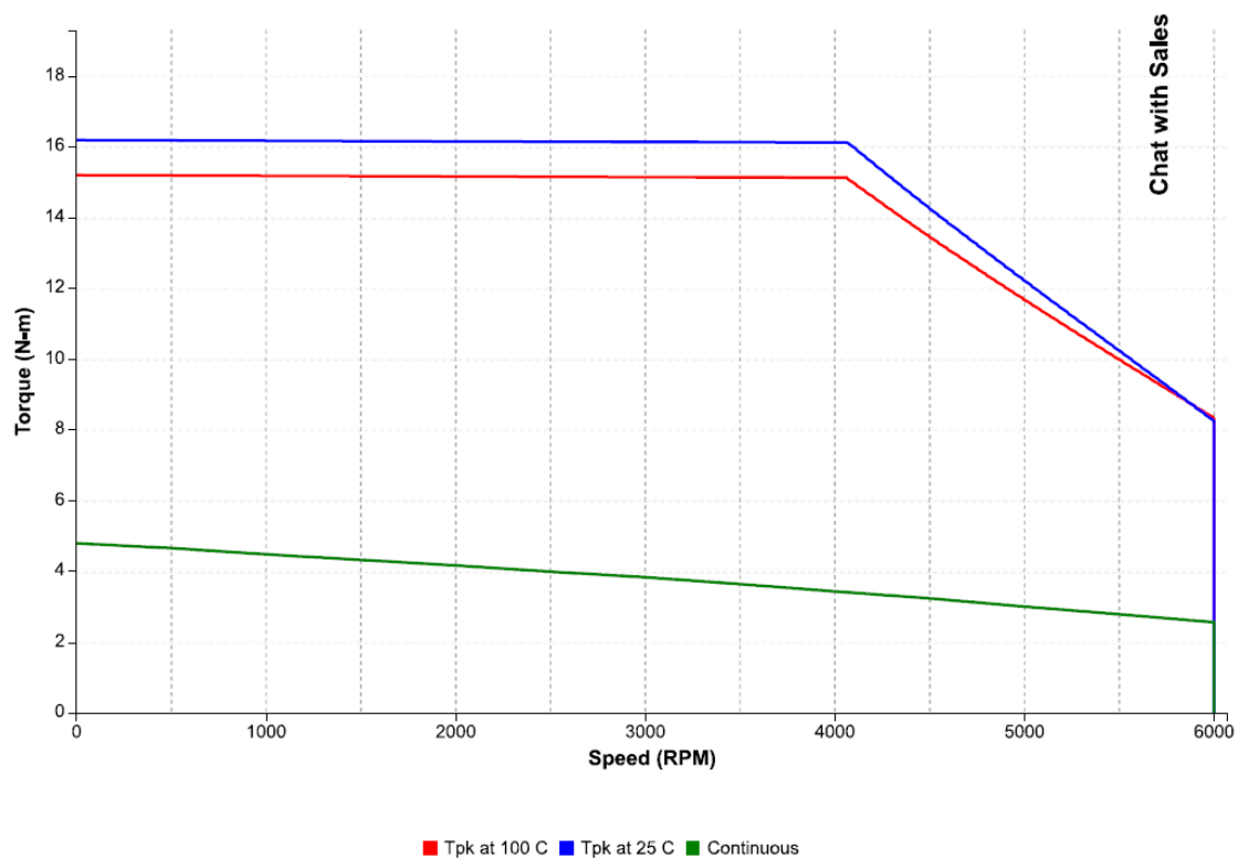
Figure 43: Speed-torque performance of an IC830M43G motor with an IC830DP00607 drive at 480 VAC
