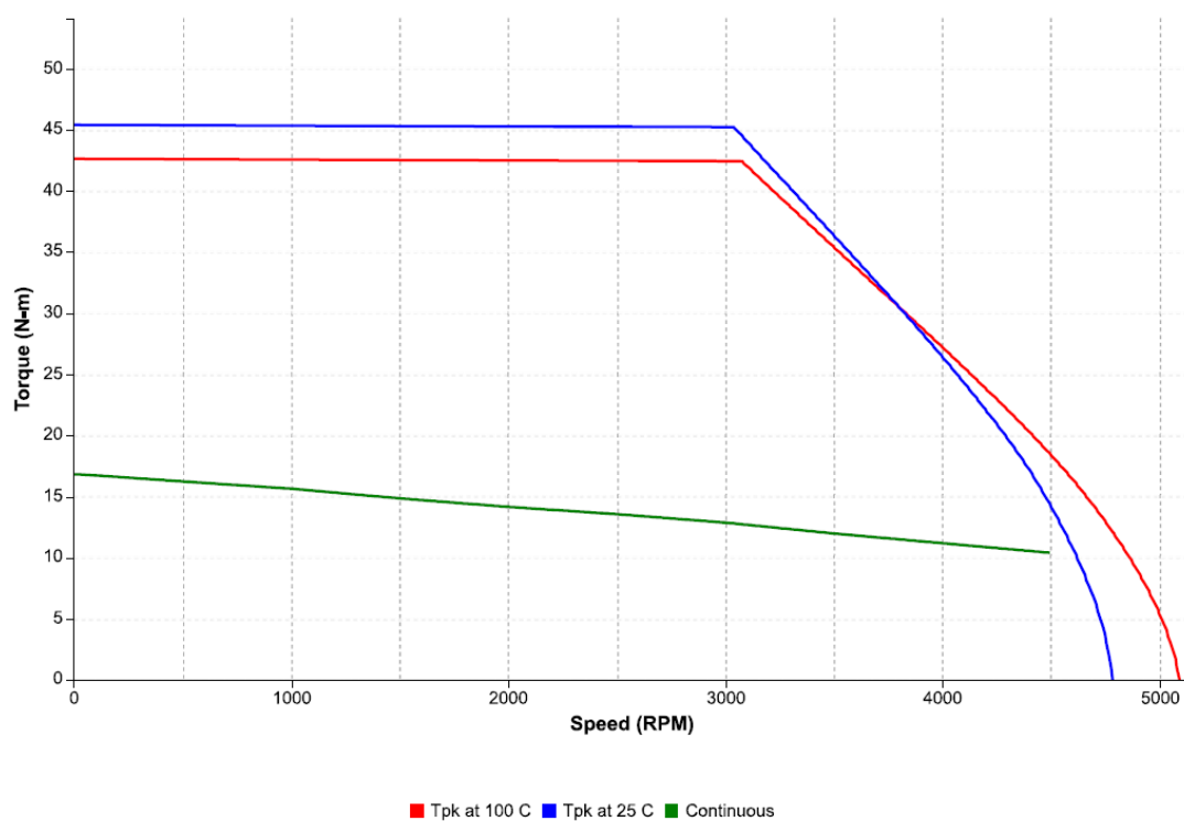
Figure 66: Speed-torque performance of an IC830M63L motor with an IC830DP02407 drive at 480 VAC
