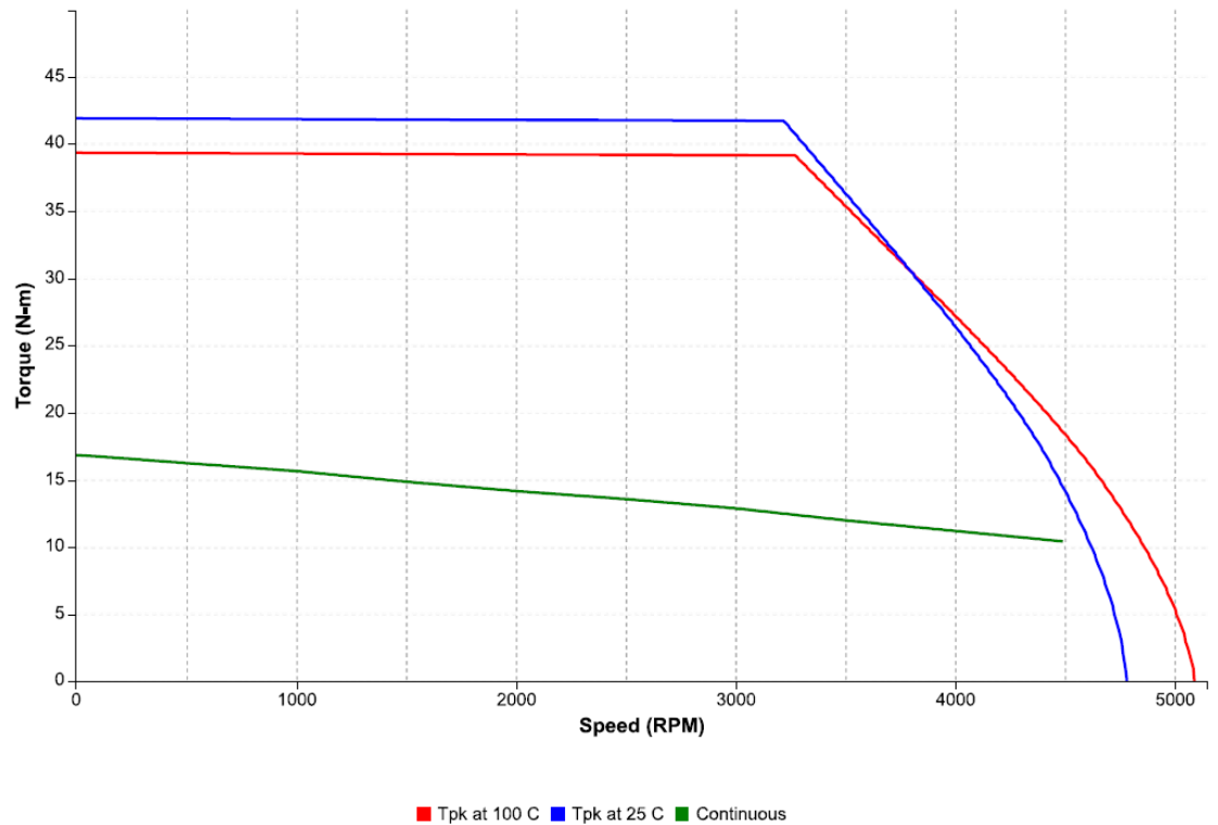
Figure 65: Speed-torque performance of an IC830M63L motor with an IC830DP01207 drive at 480 VAC
