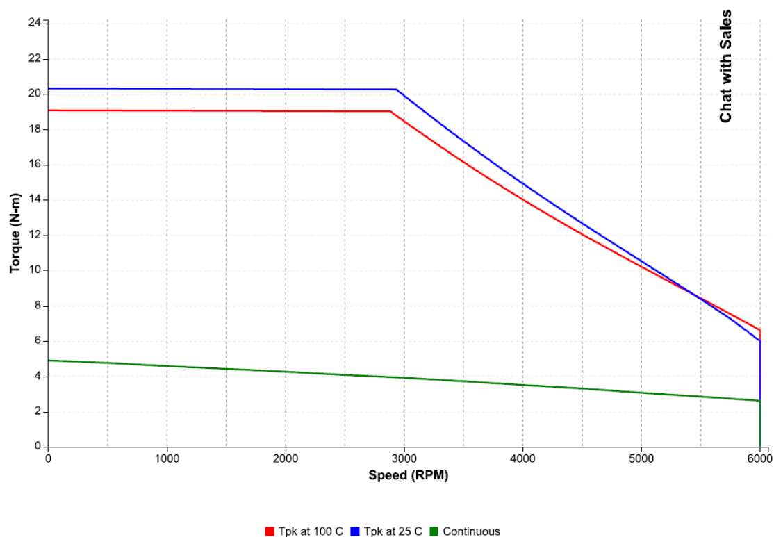
Figure 46: Speed-torque performance of an IC830M43K motor with an IC830DP02406 drive at 230 VAC
