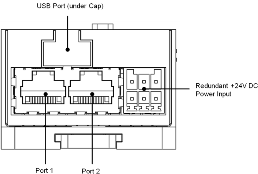
Figure 7: PROFINET Connection
