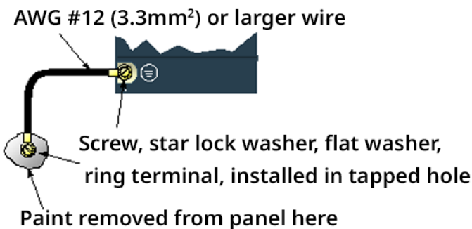
Figure 5: Ground Shield Connection
