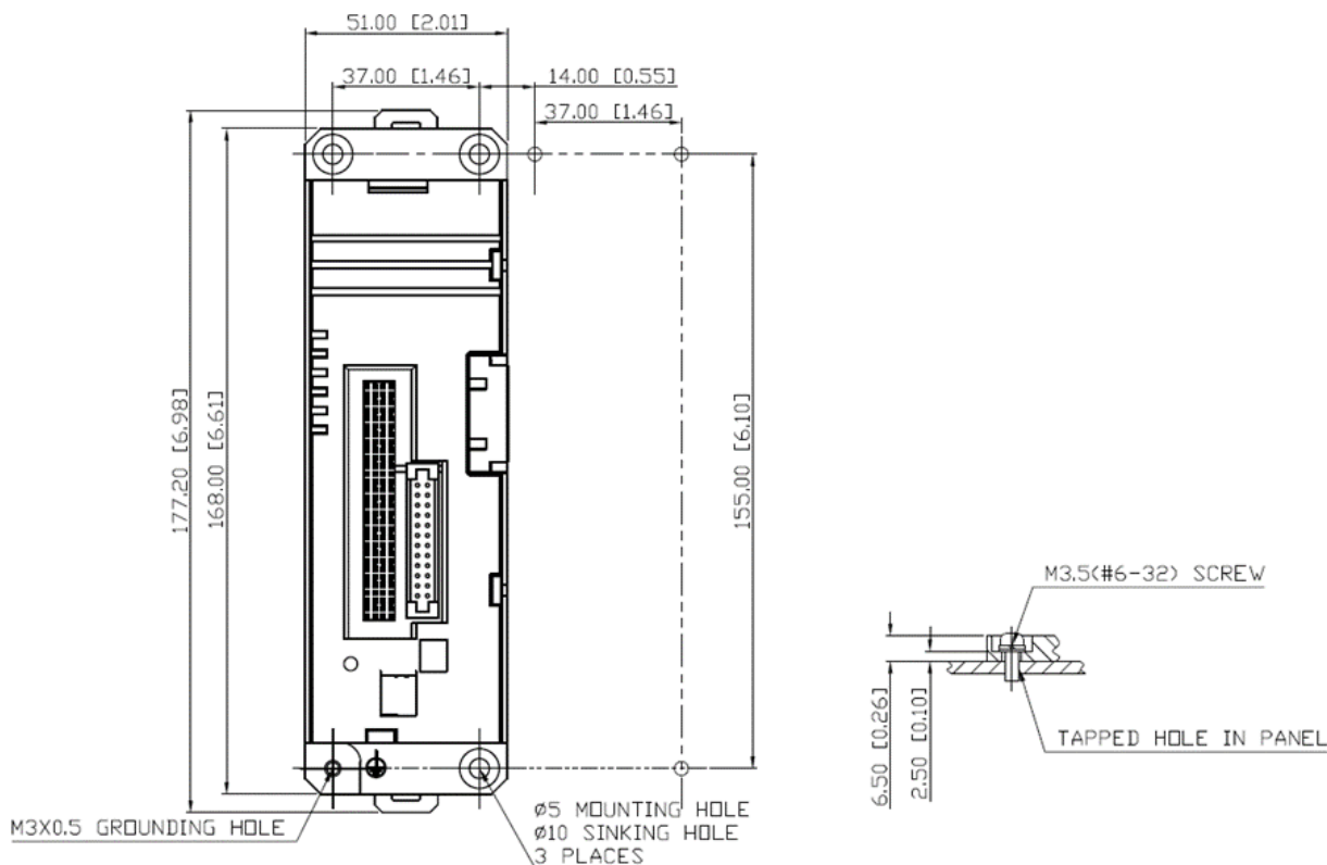
Figure 4: Panel Mounting
