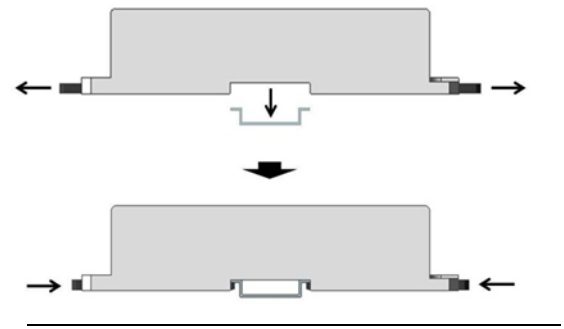
Figure 3: Installing on DIN Rail
