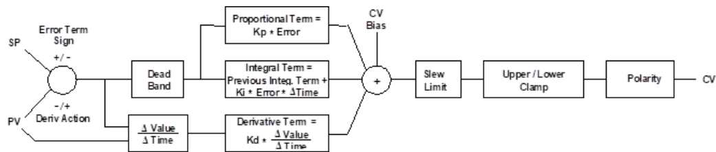
Figure 258: PID_IND Diagram
