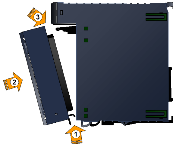
Figure 30: Installing Terminal Block into I/O Module
