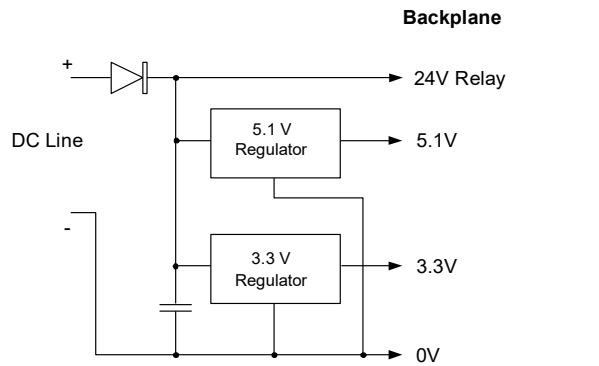
Figure 78: Outputs of Power Supply IC695PSD040 & IC695PSD140
