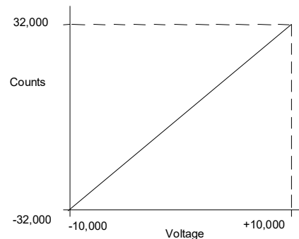
Figure 289: Scaling Example ALG608 or ALG616
