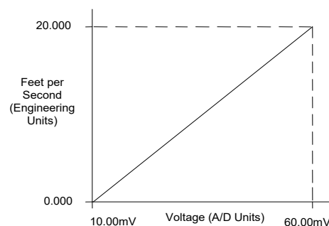
Figure 357: Input Scaling Example 1
