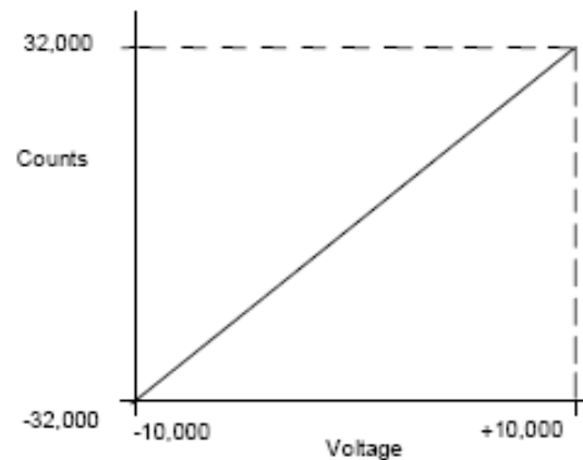
Figure 344: Output Scaling Example ALG542
