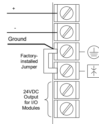
Figure 115: Field Wiring for PWR331
