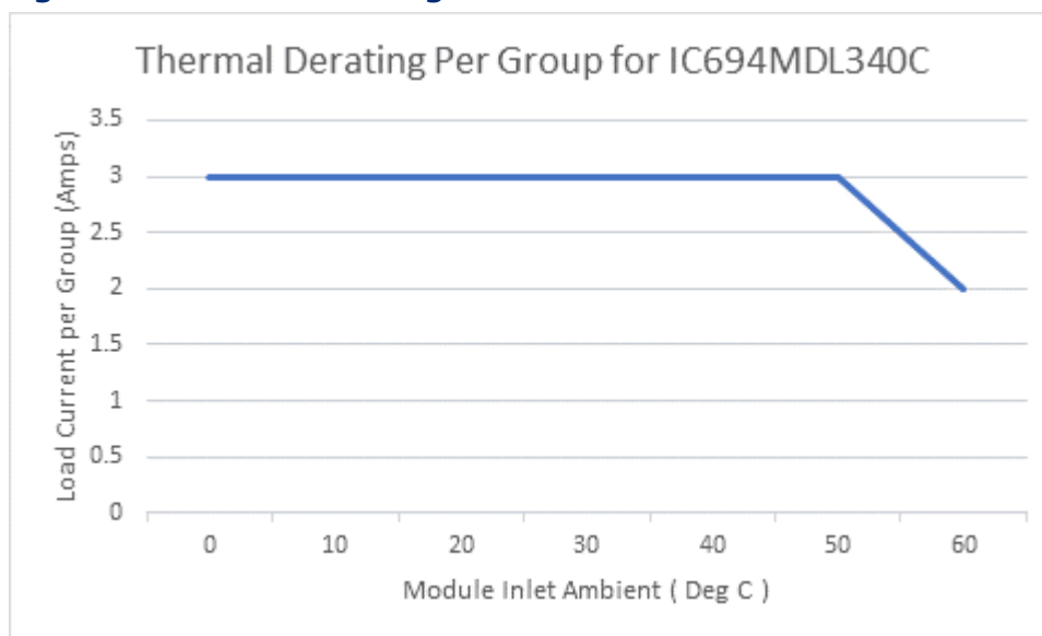
Figure 181: Thermal Derating IC694MDL340C
