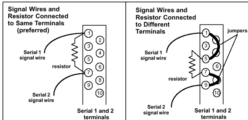
Figure 371: Installing Genius Bus Terminating Resistor
