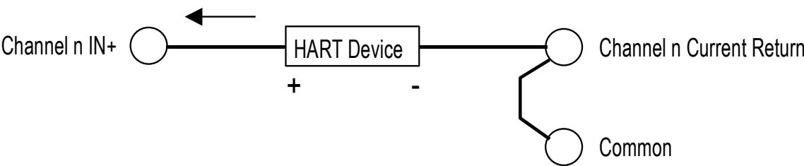
Figure 321: HART Active Source Device Connection
