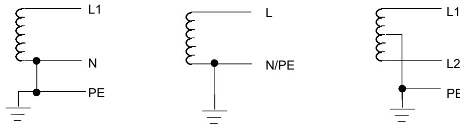
Figure 54: Neutral Not Floating (Tied to Ground)
