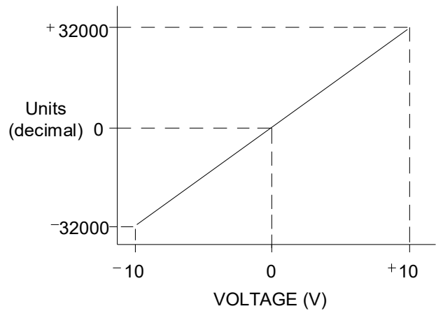
Figure 294: Scaling Units versus Output Voltage
