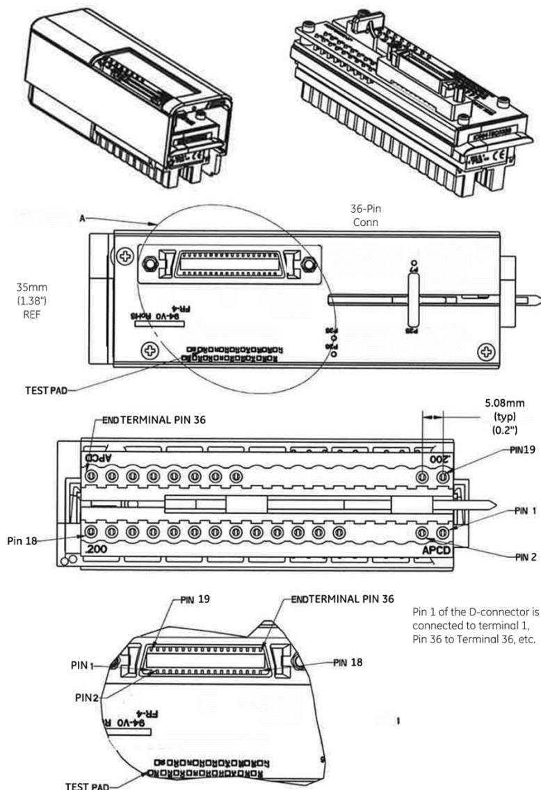
Figure 452: IC694TBC032 High-Density Terminal Block with Single 36-Pin D Connector
