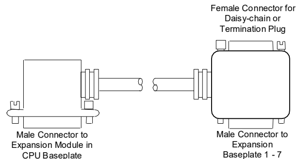
Figure 121: Cables IC693CBL300, IC693CBL301, IC693CBL312, or IC693CBL313
