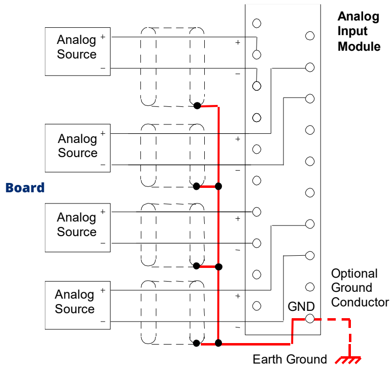
Figure 39: Analog Input Shields Connected to Module Terminal
