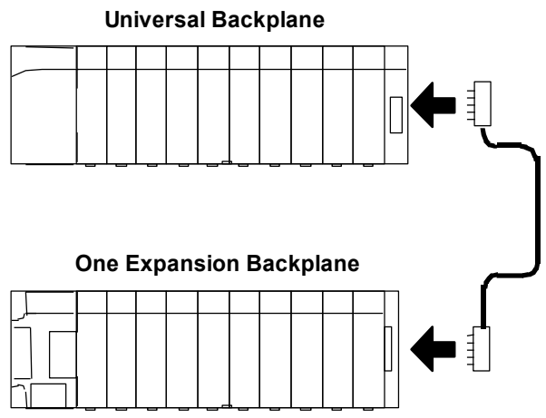
Figure 120: Cable IC693CBL302 Usage
