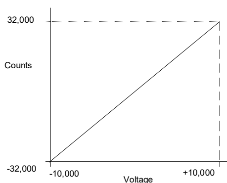
Figure 352: Input Scaling Example 2: ALG600
