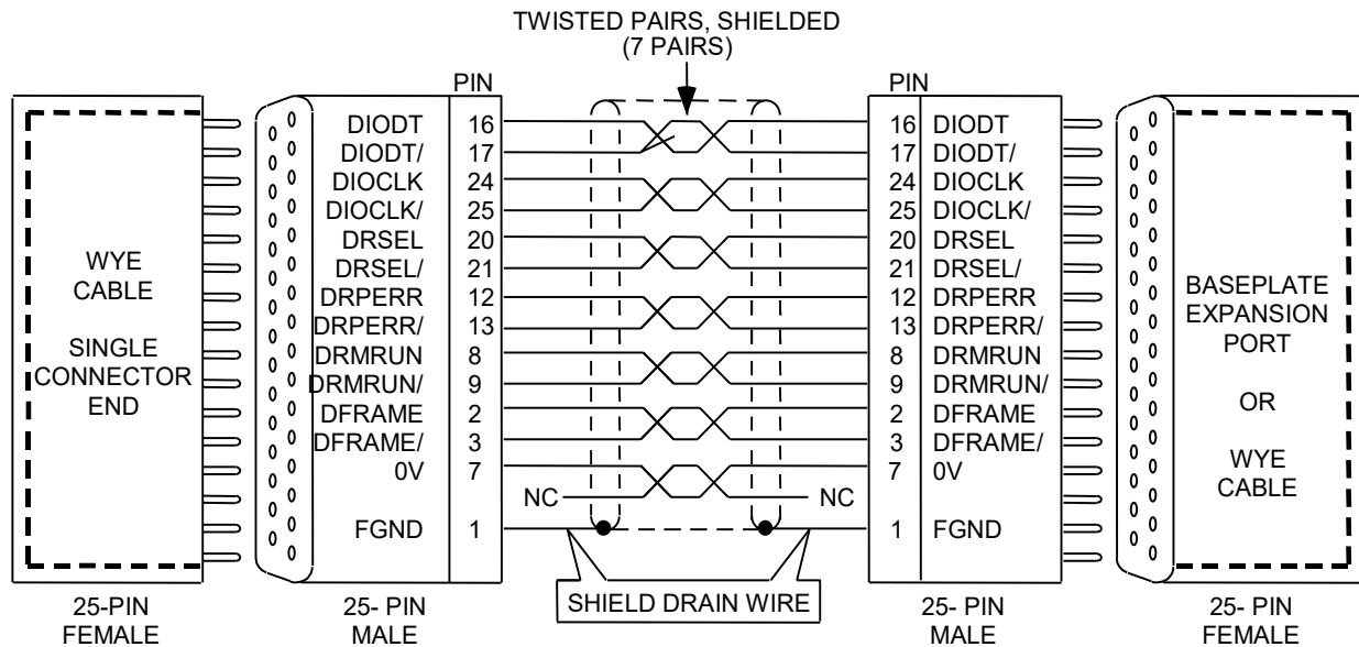
Figure 125: Wiring Diagram – Cable without Continuous Shielding
