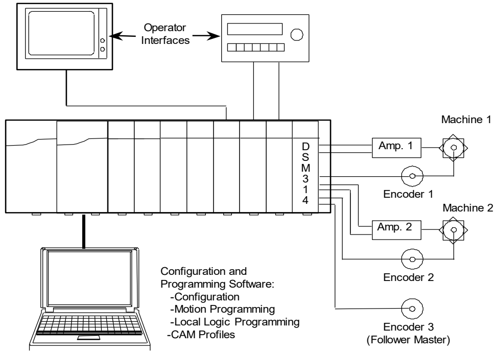
Figure 390: System Overview: DSM314
