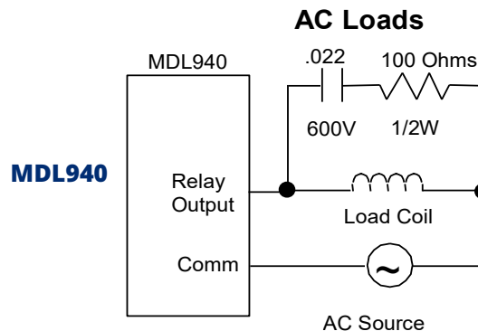
Figure 239: Suppression of AC Loads
