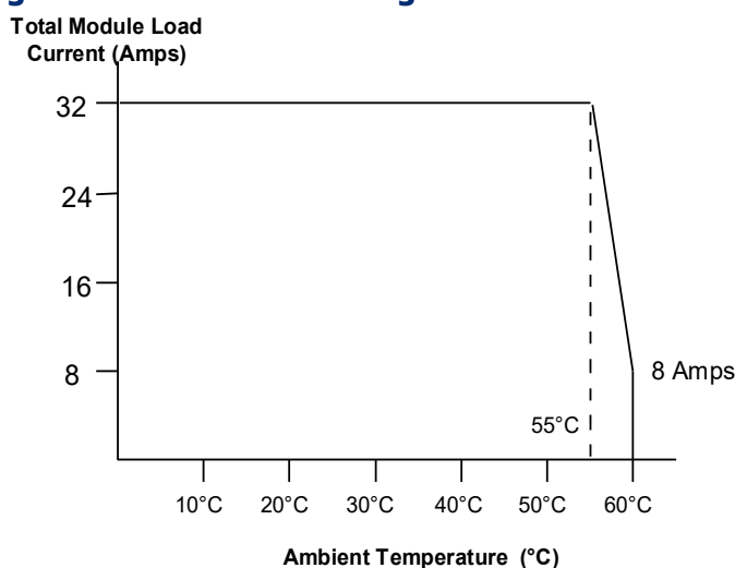
Figure 228: Thermal Derating Curve MDL930
