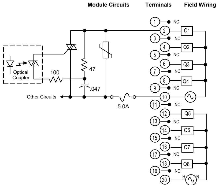
Figure 179: Field Wiring MDL330
