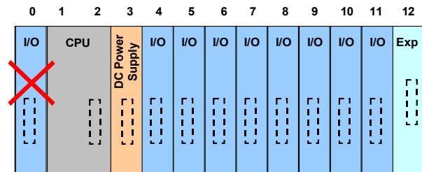
Figure 68: Invalid: Only a Power Supply can be installed in Slot
