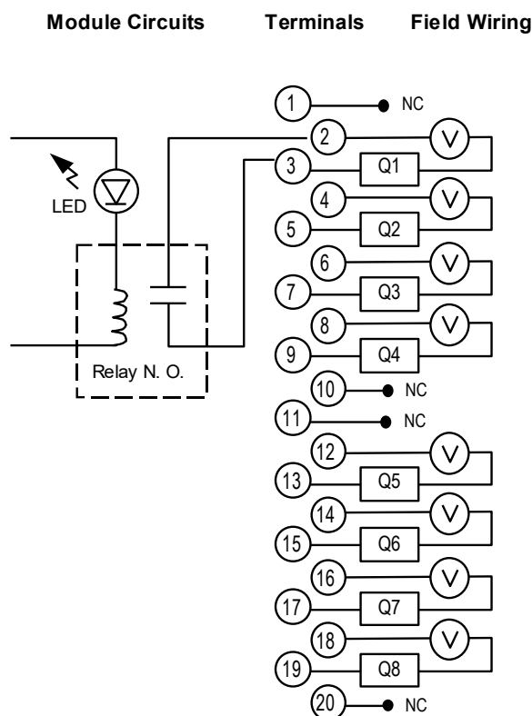
Figure 231: Field Wiring MDL930
