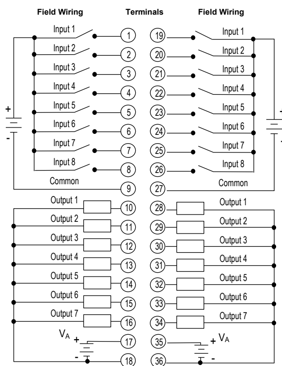
Figure 251: Field Wiring HSC304
