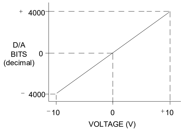
Figure 293: D/A Bits versus Output Voltage
