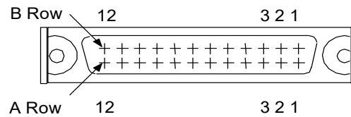
Figure 444: D-Connector Pinout
