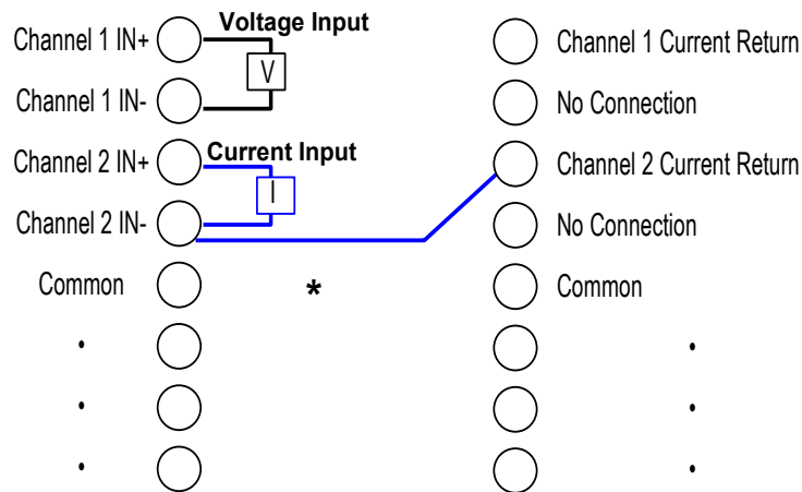
Figure 319: Field Wiring Differential Mode ALG626 or ALG628
