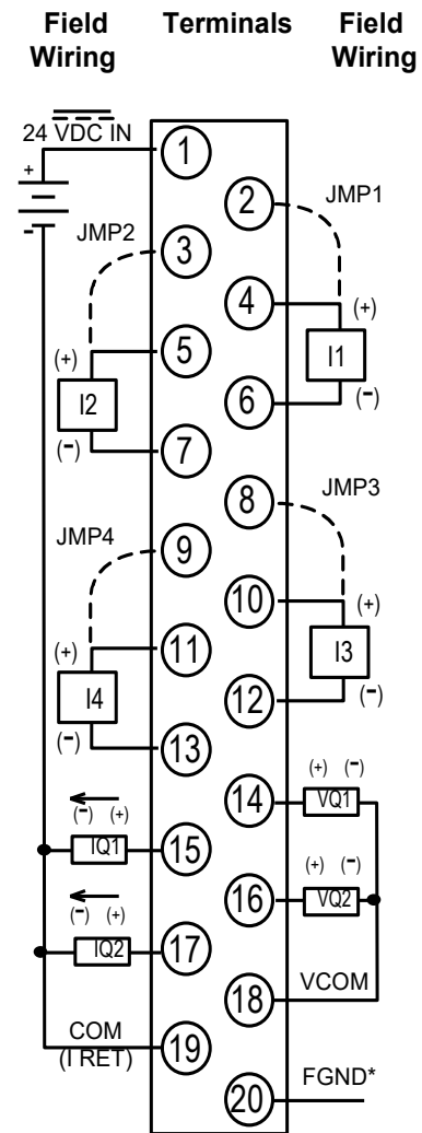
Figure 342: Field Wiring ALG542
