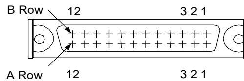
Figure 444: D-Connector Pinout
