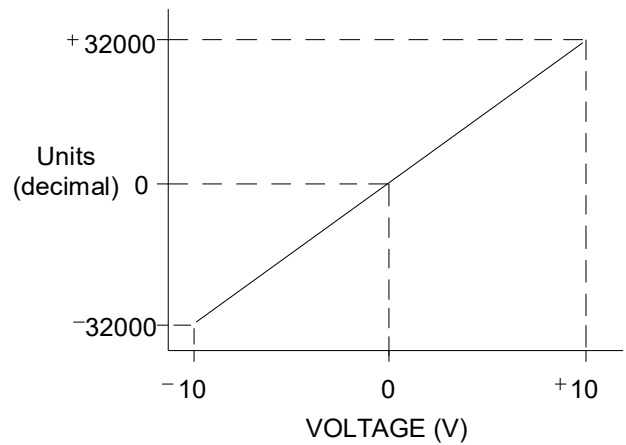
Figure 294: Scaling Units versus Output Voltage
