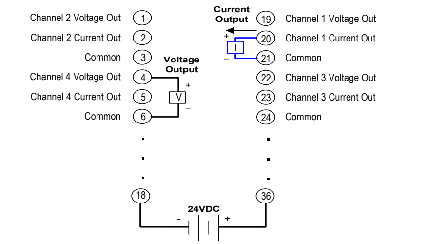
Figure 309: Field Wiring ALG704 & ALG708
