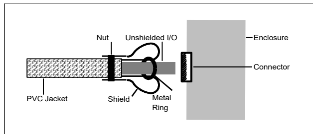
Figure 454: Unshielded I/O Cable, Single Shield (Side View)
