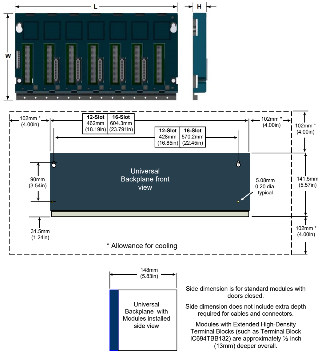
Figure 9: RX3i Universal Backplane Dimensions and Spacing
