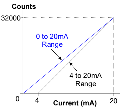
Figure 337: Output Current Scaling ALG442
