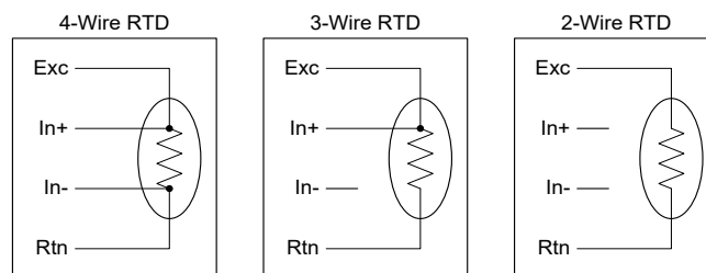
Figure 360: Field Wiring for RTDs ALG508
