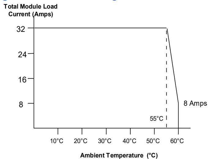
Figure 228: Thermal Derating Curve MDL930
