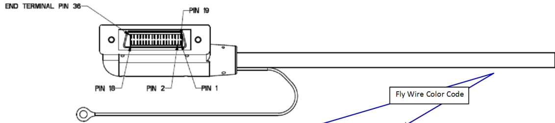
Figure 453: IC694CBL* Cable Wiring Details
