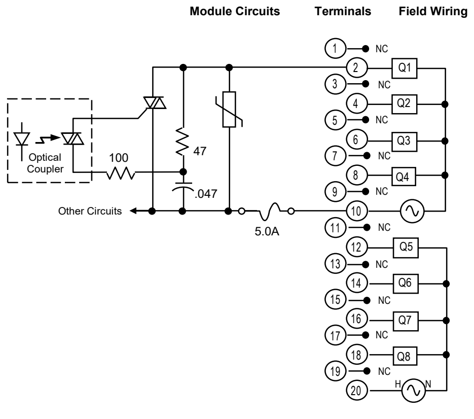
Figure 179: Field Wiring MDL330
