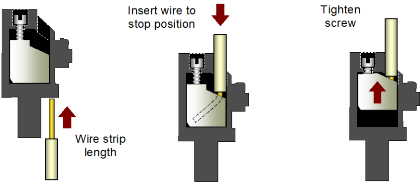
Figure 428: Wire Preparation and Insertion into Box-Style Terminal Block
