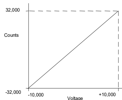
Figure 317: Scaling Example ALG626/ALG628
