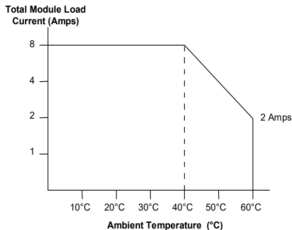
Figure 178: Thermal Derating Curve MDL330
