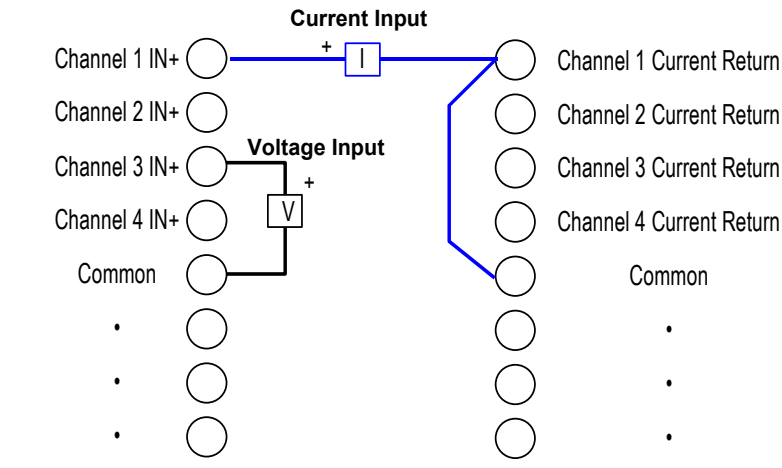
Figure 318: Field Wiring Single-Ended ALG626 or ALG628
