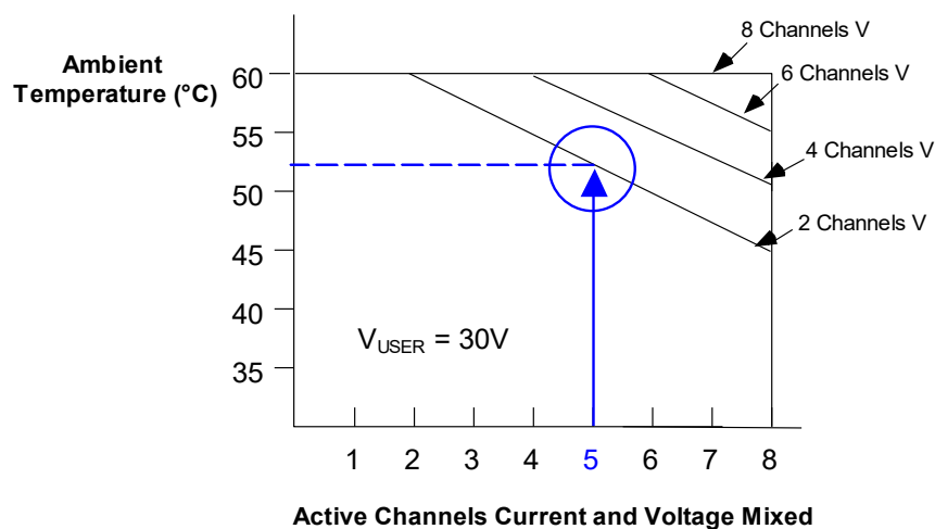
Figure 302: Derating for Mixed Current & Voltage Outputs: ALG392
