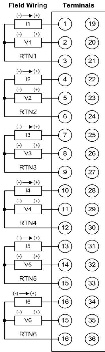
Figure 258: Field Wiring ALG106
