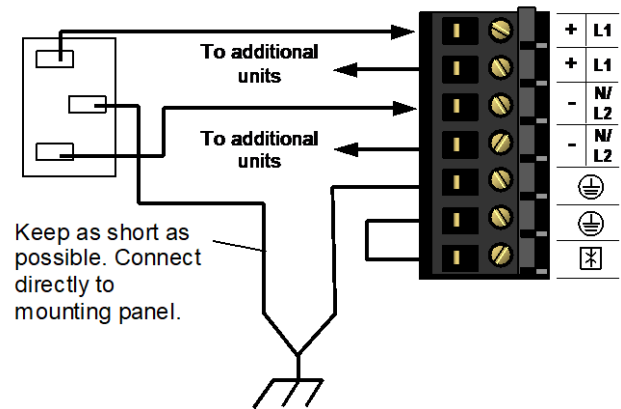
Figure 94: Field Wiring for PSA140
