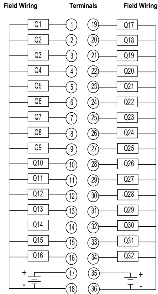
Figure 212: Field Wiring MDL754
