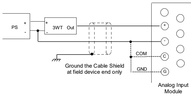
Figure 42: 3-Wire Transducer, Externally Powered by DC Supply
