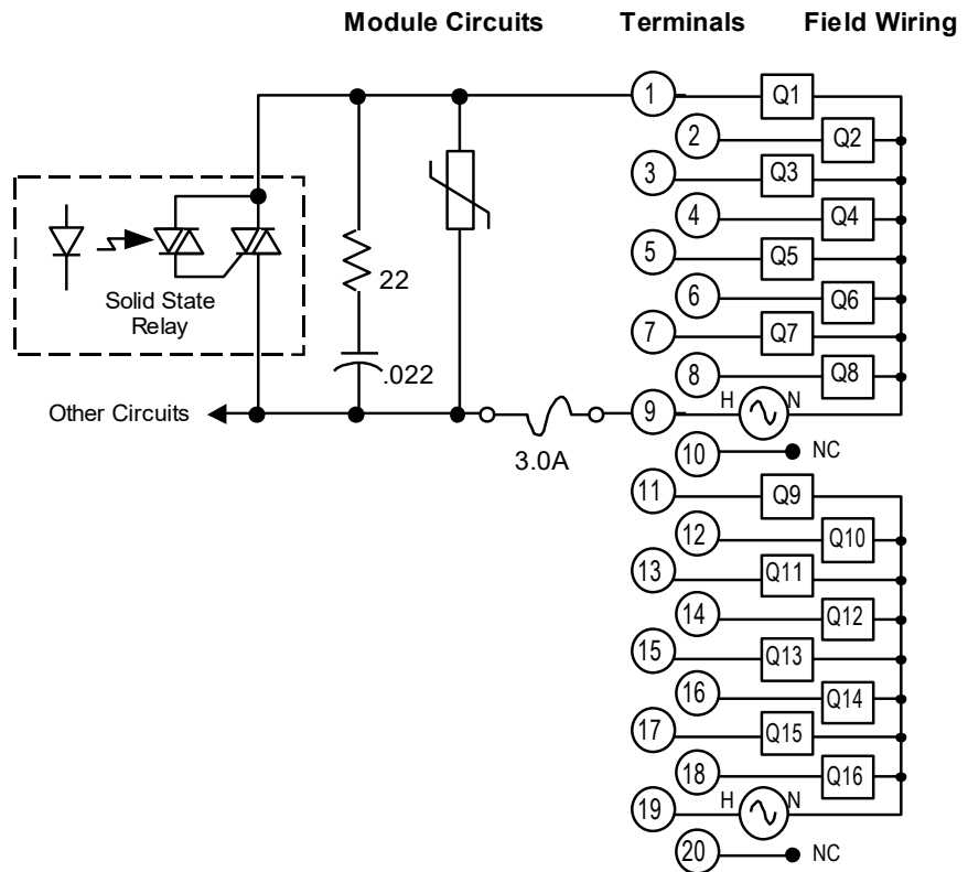
Figure 182: Field Wiring MDL340
