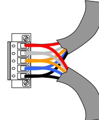
Figure 388: DeviceNet Wiring for Daisy Chain
