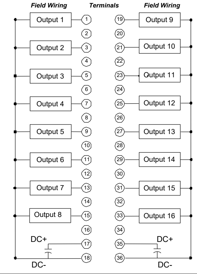
Figure 219: Field Wiring MDL765
