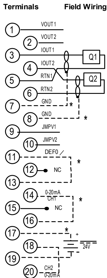
Figure 298: Field Wiring ALG391
