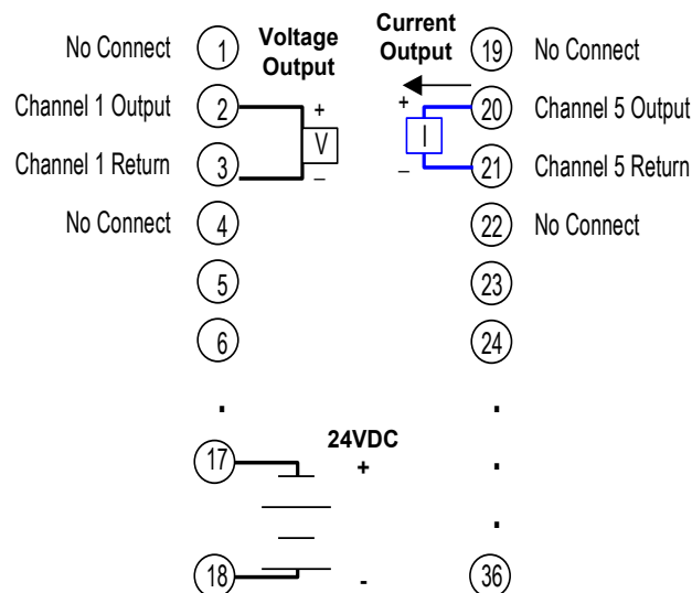
Figure 312: Field Wiring: ALG808
