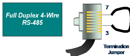
Figure 378: Using External Jumper & Built-in 120Ω Resistor for RS-485 4-Wire Full Duplex
