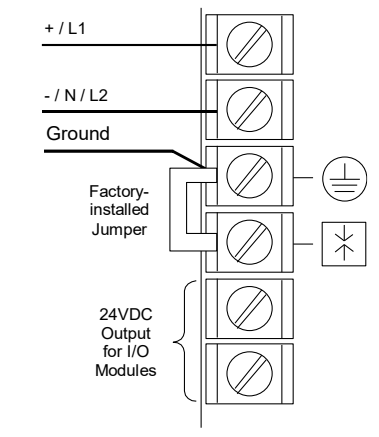
Figure 111: Field Wiring for PWR330
