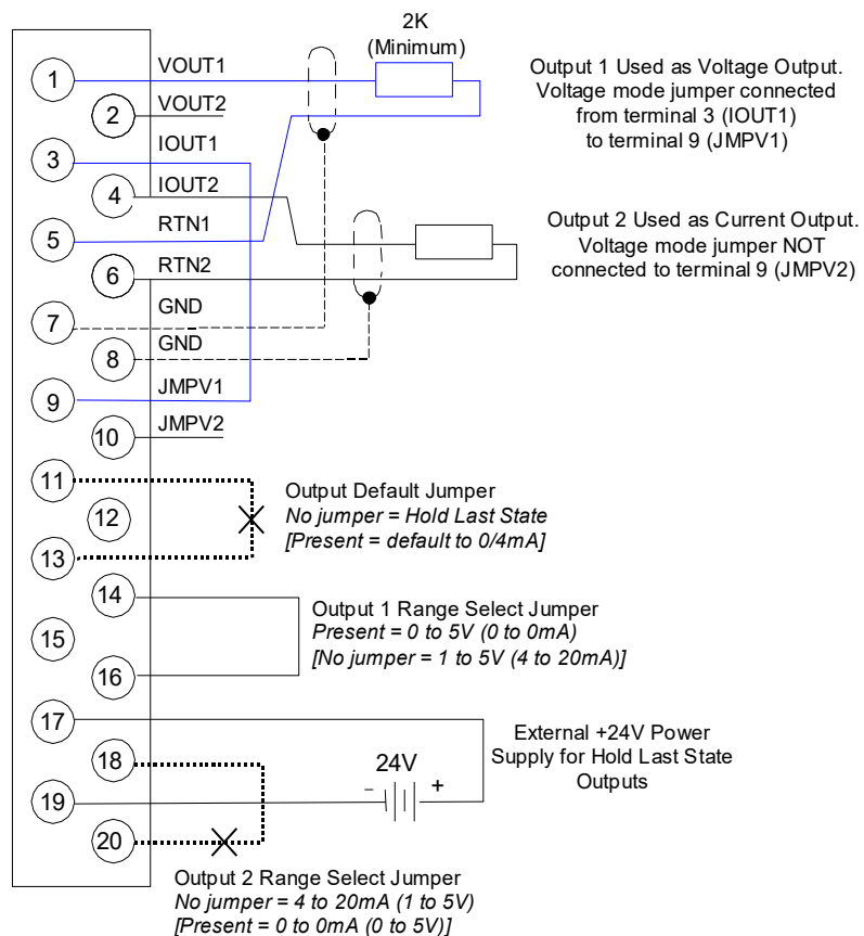
Figure 299: Wiring Example ALG391
