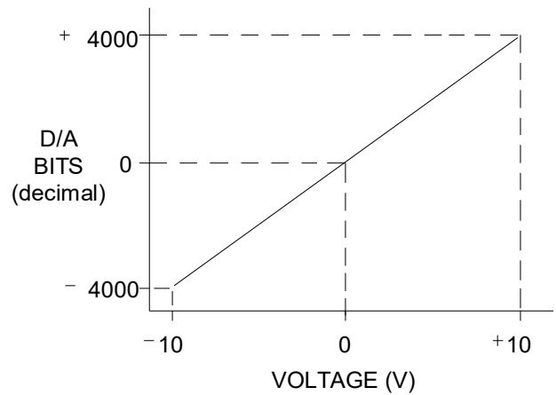
Figure 293: D/A Bits versus Output Voltage
