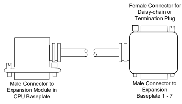
Figure 121: Cables IC693CBL300, IC693CBL301, IC693CBL312, or IC693CBL313
