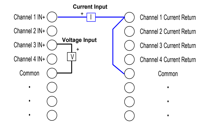
Figure 290: Field Wiring, Single-Ended ALG608 or ALG616
