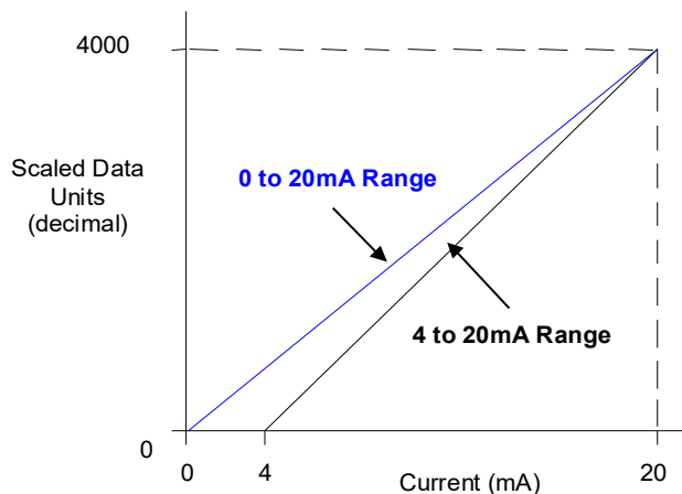
Figure 273: Input Scaling ALG223
