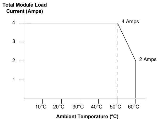
Figure 175: Thermal Derating Curve MDL310
