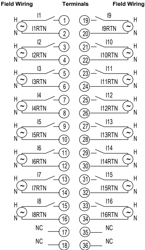
Figure 136: Field Wiring MDL250
