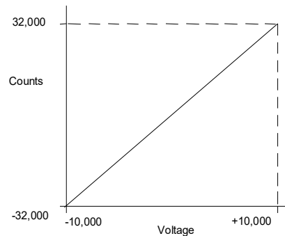
Figure 311: Channel Scaling Example
