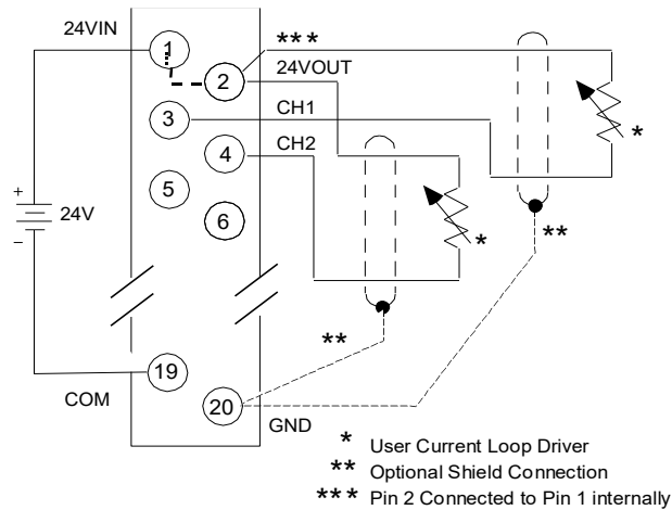
Figure 275: Connection Example 1 ALG222
