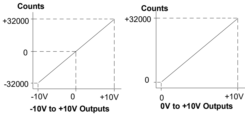
Figure 336: Output Voltage Scaling ALG442
