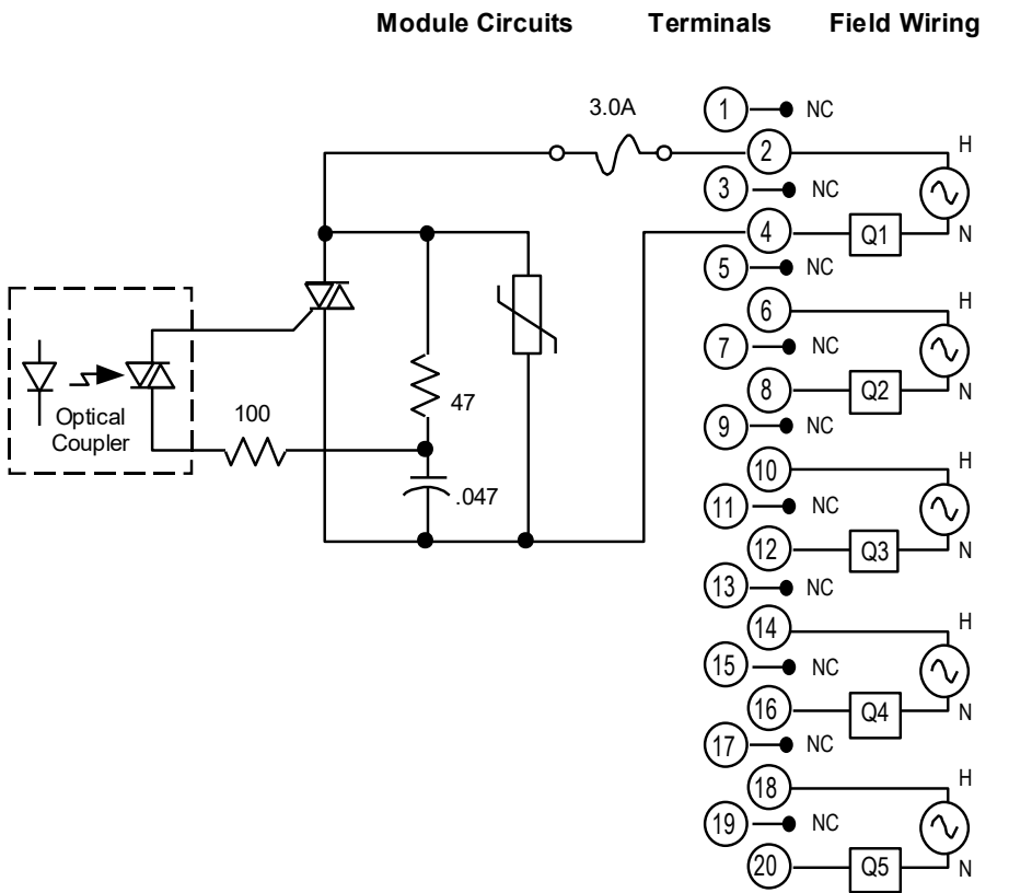
Figure 188: Field Wiring MDL390
