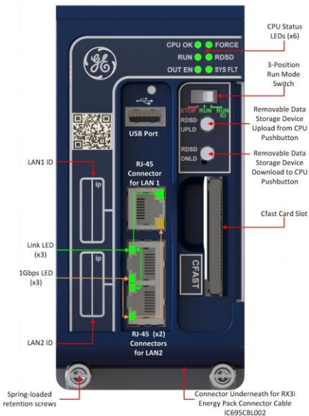
Figure 1: IC695CPE330 Features at a Glance
