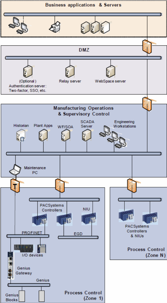
Figure 1: Reference Architecture
