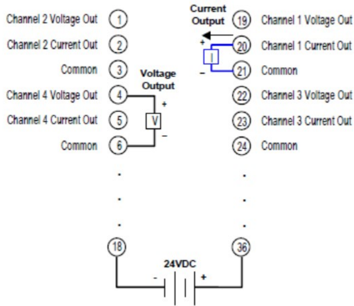
Figure 3: Field Wiring
