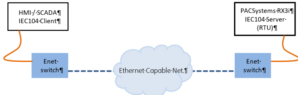
Figure 1 : IEC 104 Basic System Architecture
