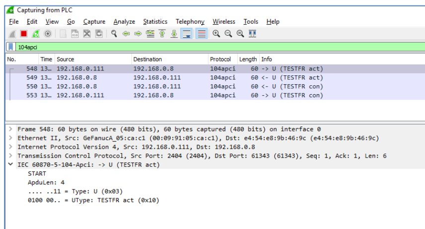
Figure 35:Wire Shark Trace for Control Commands
