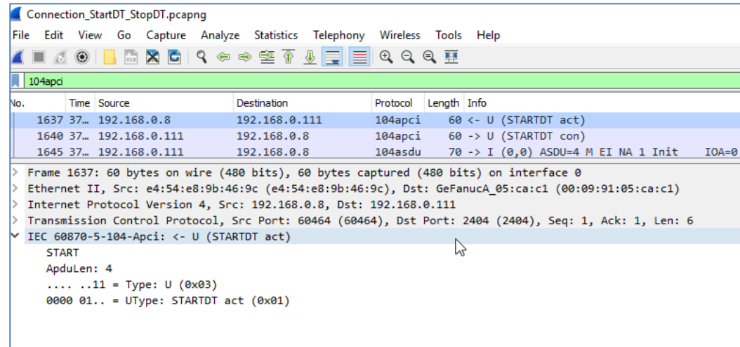
Figure 33: Wireshark Trace of STARTDT Function
