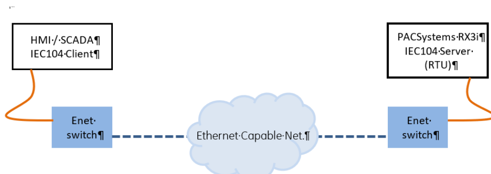
Figure 1 : IEC 104 Basic System Architecture
