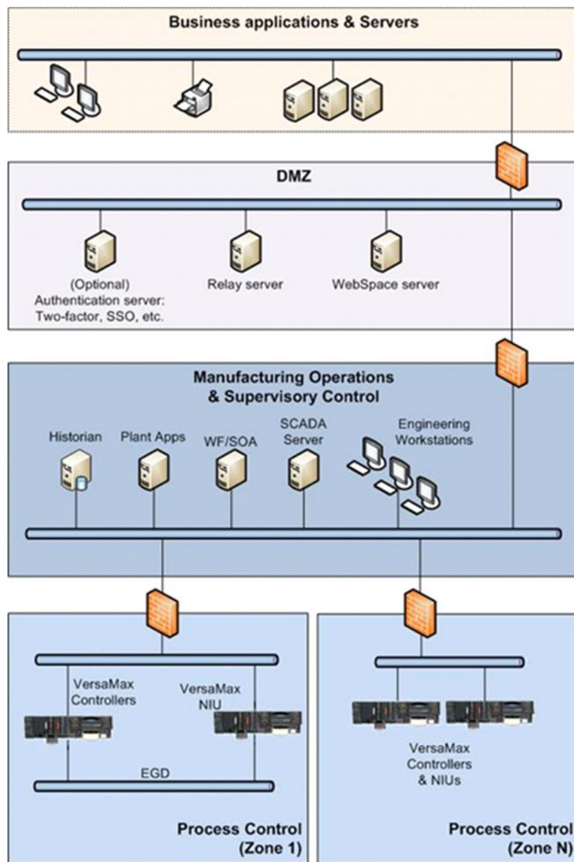
Figure 6-1: Reference deployment of VersaMax controllers
