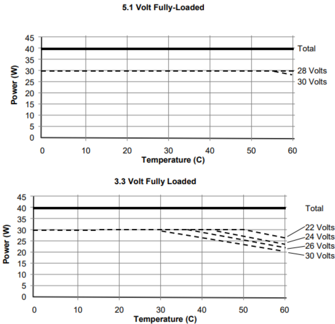
Figure 3: Thermal Derating
