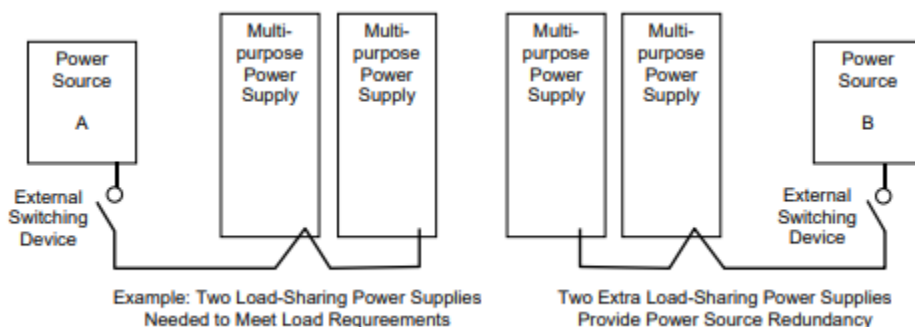
Figure 9: Powersupply Redundancy
