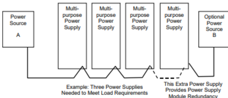
Figure 8: Powersupply Redundancy
