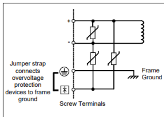
Figure 5: Over Voltage Protection
