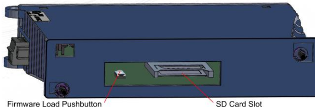
Figure 5: Rear View of Module
