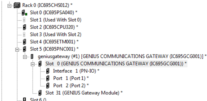
Figure 8: Configuration Steps
