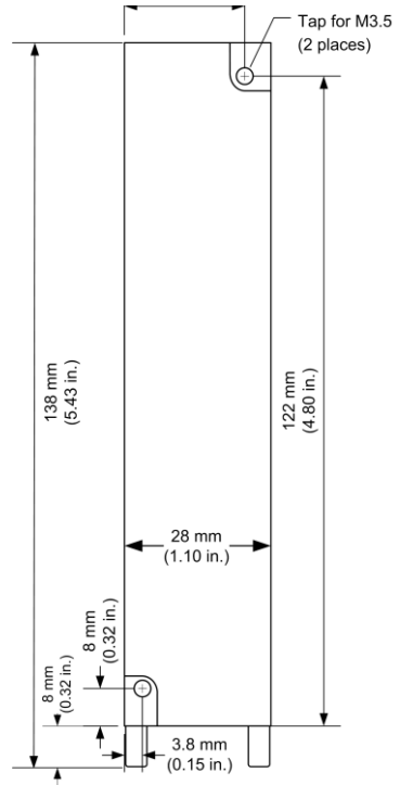
Figure 7: Panel Mounting
