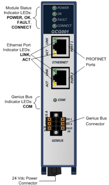
Figure 1: Module Features
