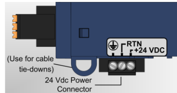
Figure 4: Power Connector
