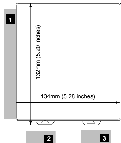
Figure 1: Module Dimension
