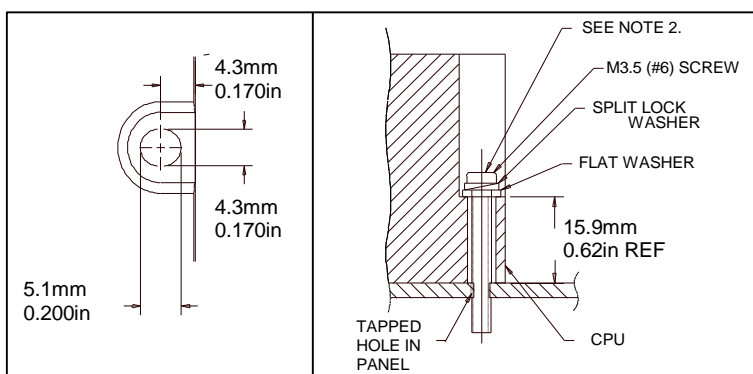
Figure 3: Panel Mounting
